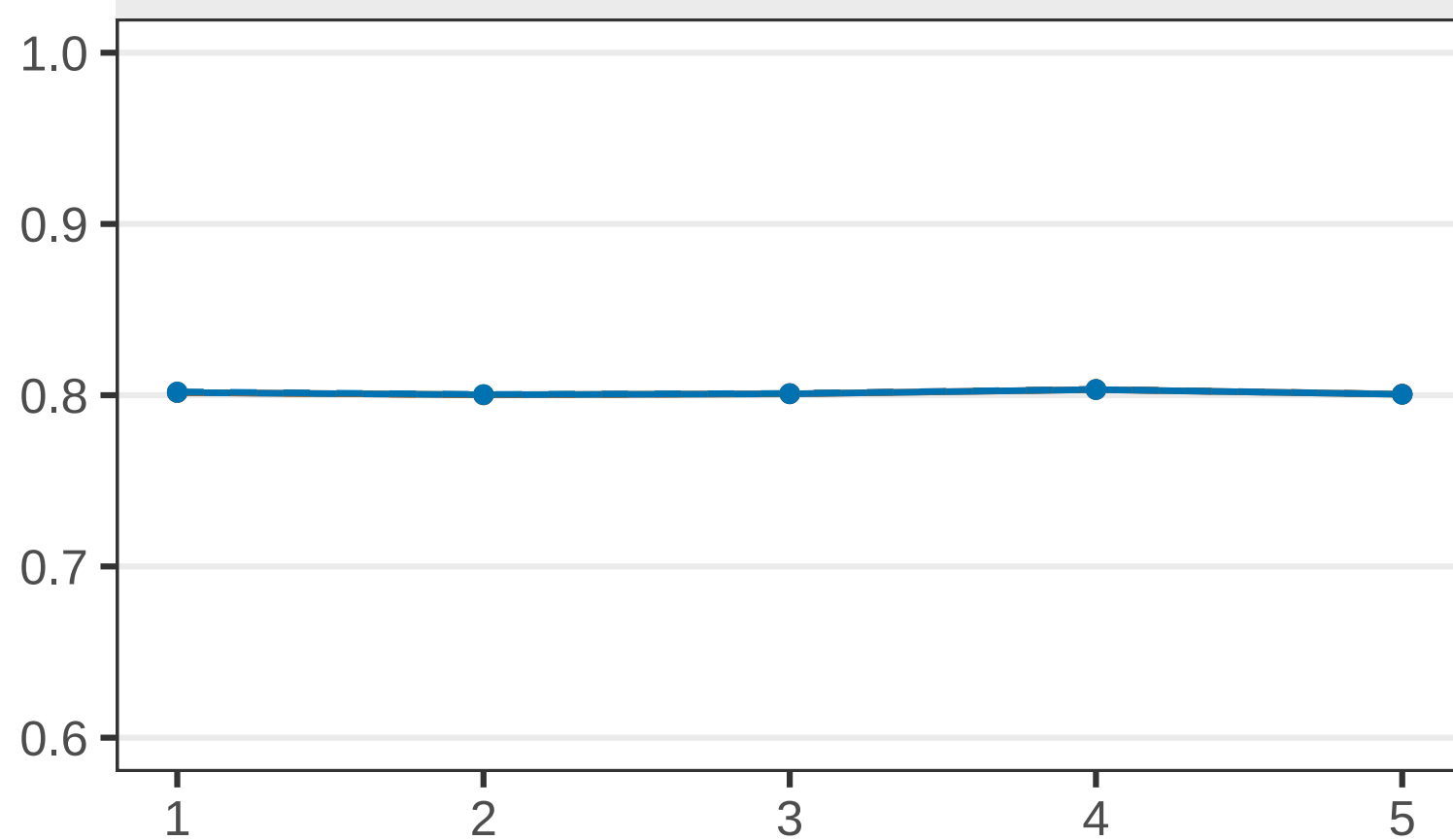
Power ( H_1 )
