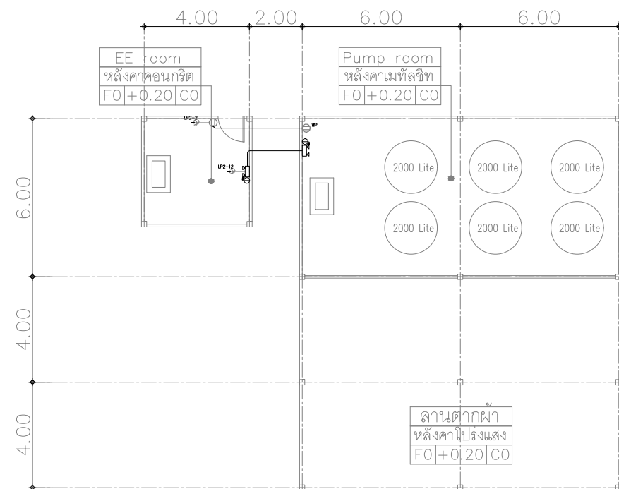
Lighting Plan EE-room, Pump room Scale 1:100
