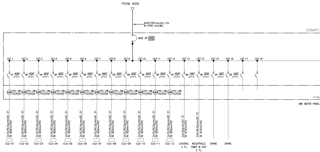
SINGLE LINE DIAGRAM MDB&DB
