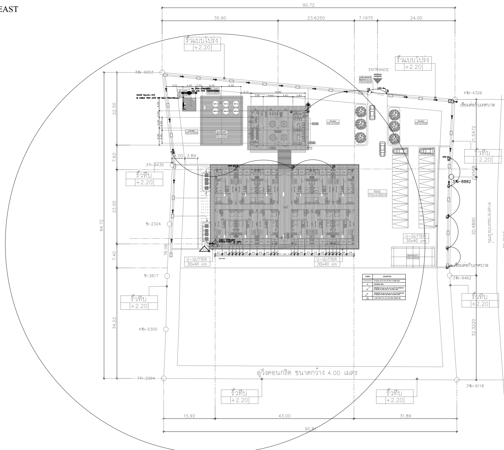
Site Plan Main Electrical & Grounding Plan — 1 st Floor
