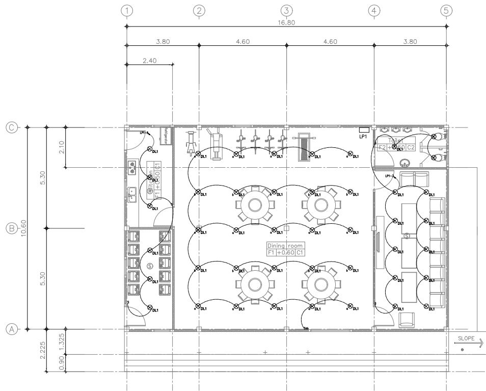
Lighting Plan DINING ROOM Scale 1:100
