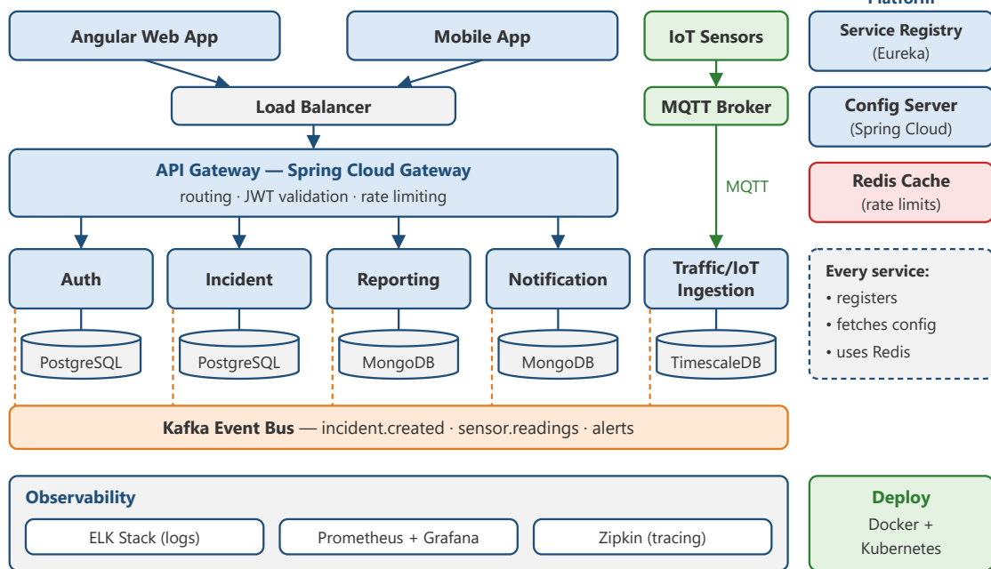
Figure 19: Smart City Microservices Reference Architecture
