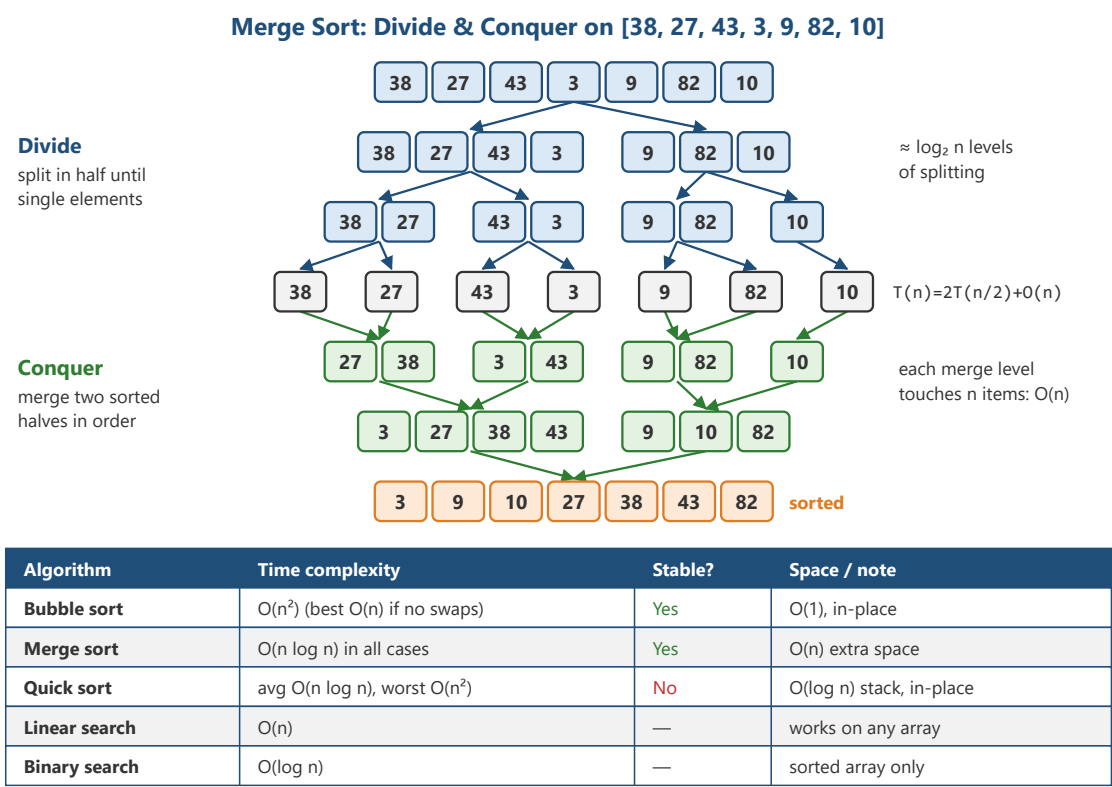
Figure 10: Merge sort divide and conquer, with sorting and searching complexities
