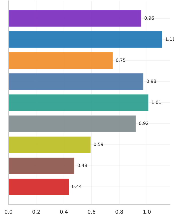
Excess Sharpe
