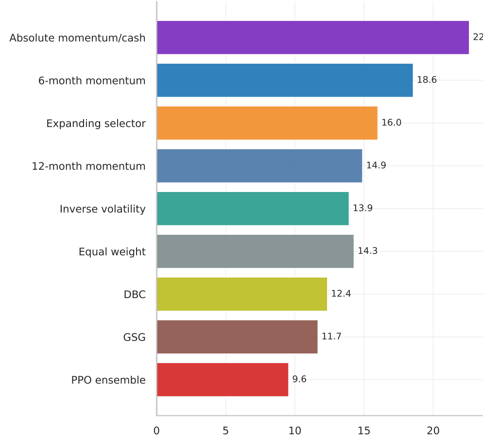
CAGR (%)
