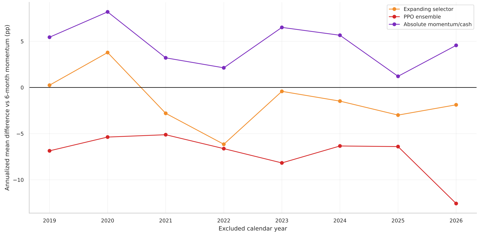
Leave-one-year-out tests reveal unstable relative performance
