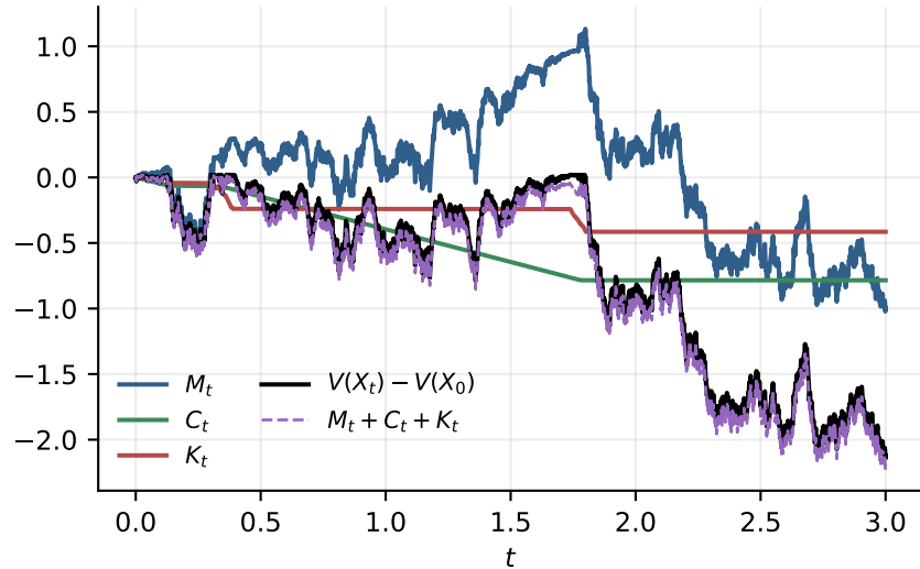
Terms for V = -x^2/2 ( x < 0 ), V = -x ( x \geq 0 )
