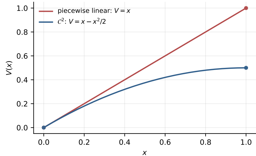
Increasing certificate candidates
