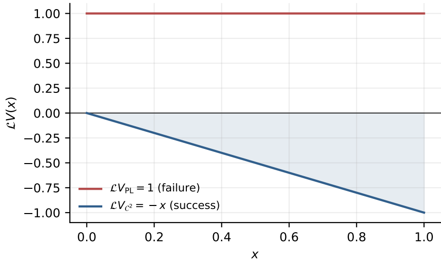
Generator for f = 1, g = \sqrt{2}
