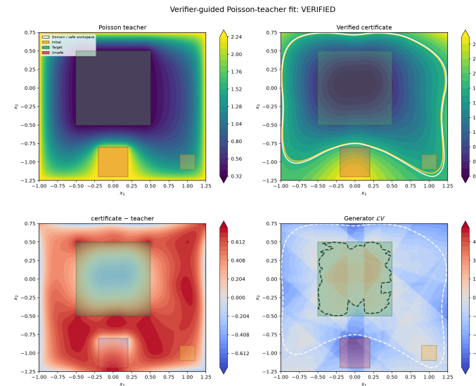
Figure 3. A verifier-guided Poisson-teacher fit: the teacher, verified certificate, approximation error, and verified generator.
