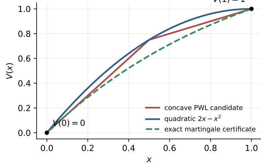
Same boundary conditions V(1) = 1
