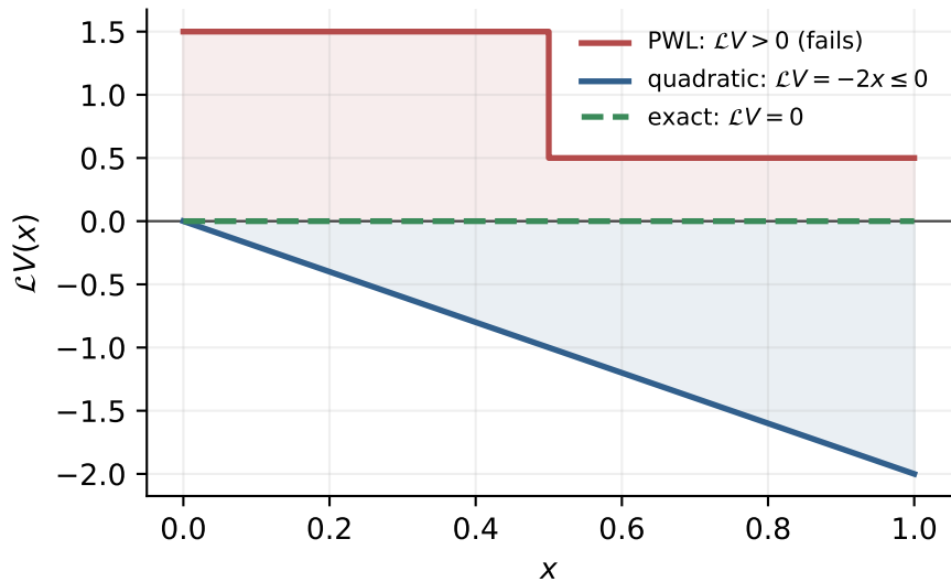
Generator for dX_t = dt + \sqrt{2} dW_t
