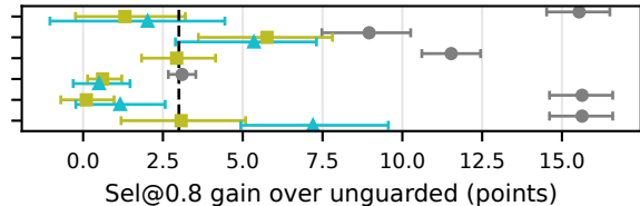
NetConfEval
