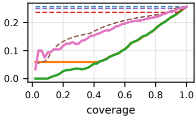
30B
