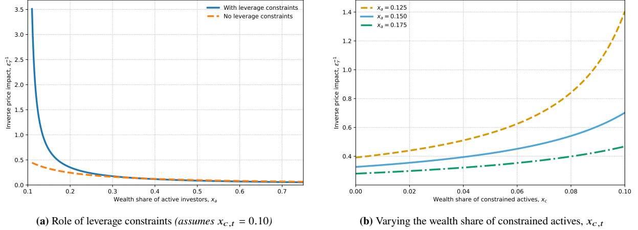
Figure 6. Price impact under binding leverage constraints. Panel (a) compares the cases with and without leverage constraints (holding x_{c,t} = 0.10 ). Panel (b) plots the price impact as a function of x_{c,t} for different values of x_{a,t} .
