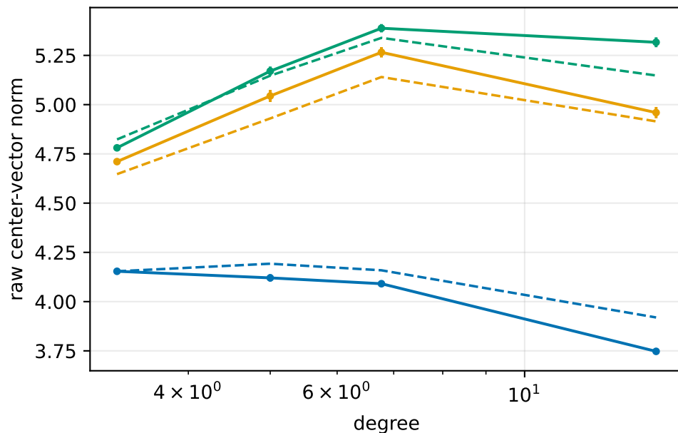
NetScience
