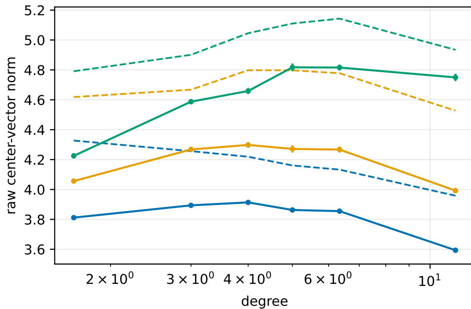
NetScience
