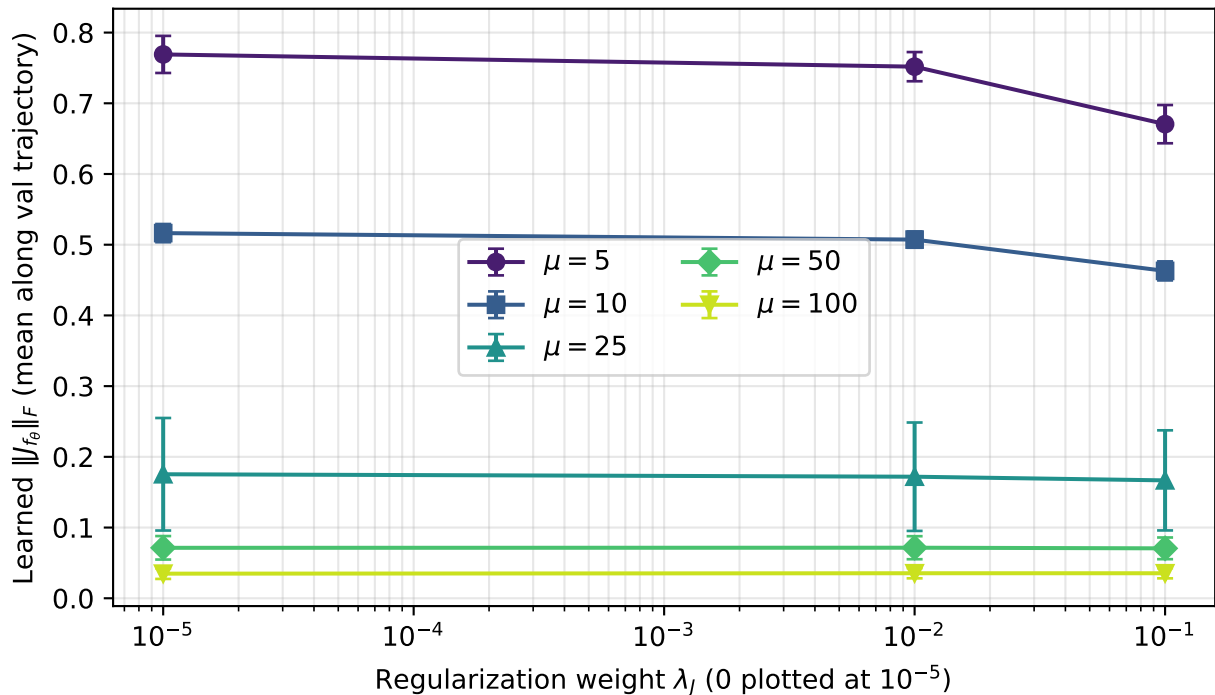
Graded Jacobian regularization engagement (Van der Pol)
