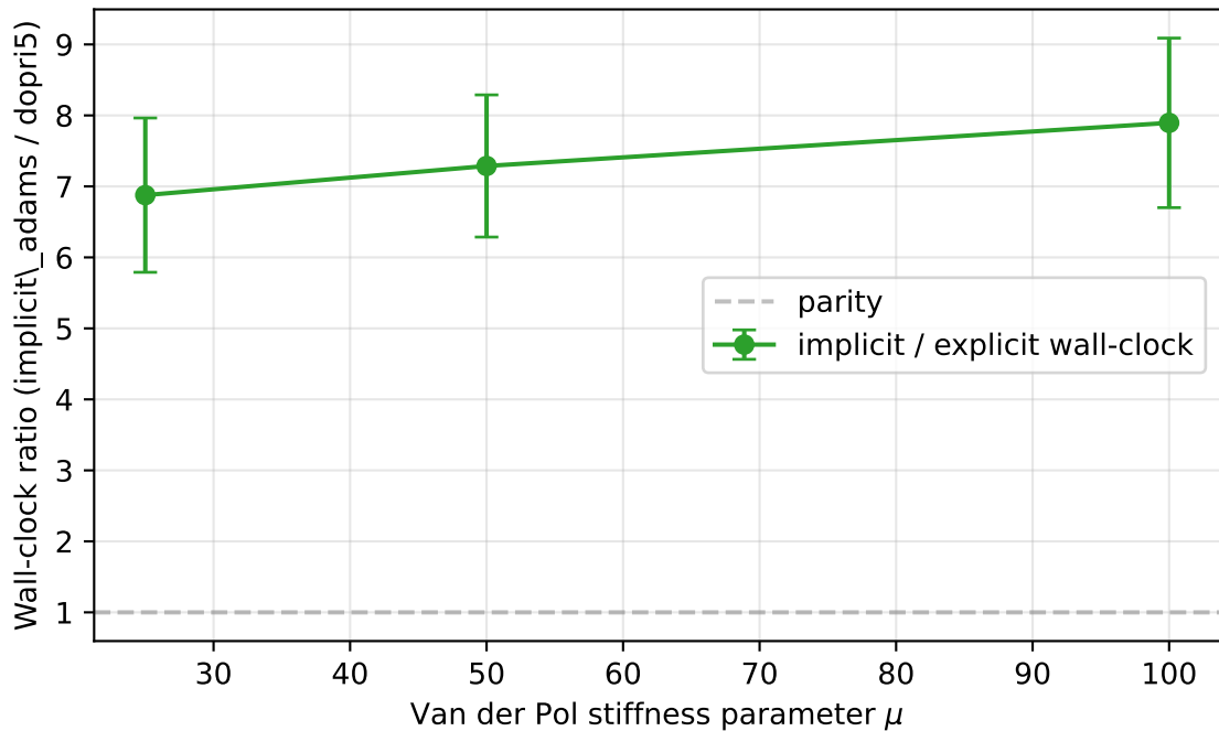
H3: Implicit advantage shrinks (ratio grows) with \mu
