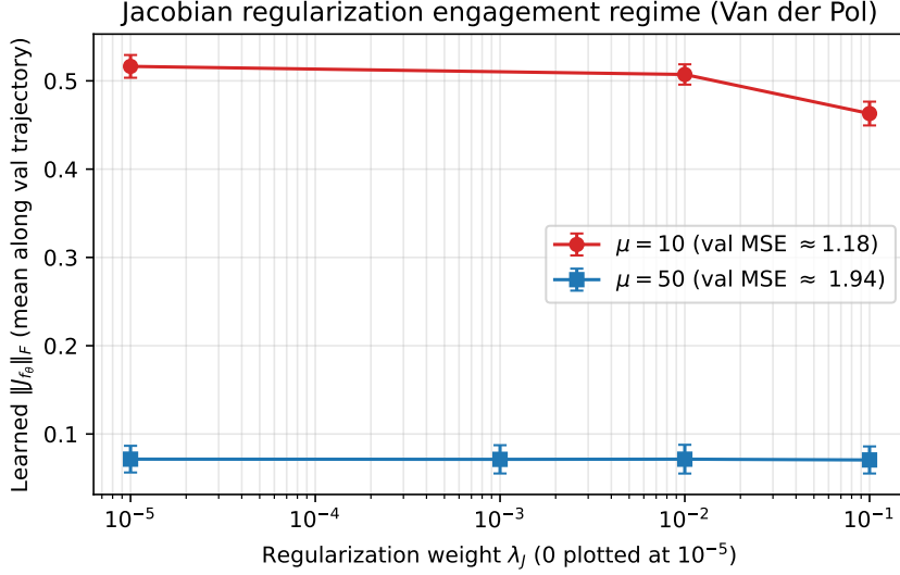
Figure 1: Engagement regime. Learned Jacobian Frobenius norm versus regularization weight \lambda_J , on Van der Pol at \mu = 10 (better-fit) and \mu = 50 (poorer-fit). Each point is the mean over 5 seeds; bars are \pm 1 std. At \mu = 10 the penalty suppresses \|J_{f_\theta}\|_F monotonically as \lambda_J increases; at \mu = 50 the curve is essentially flat.
