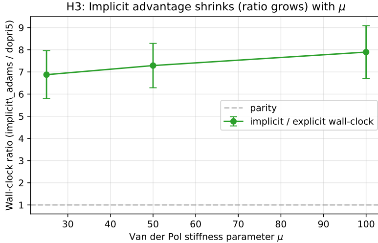
Figure 2: H3 stiffness slope. Wall-clock ratio of implicit_adams to dopri5 on Van der Pol as \mu varies. The ratio grows monotonically, meaning the explicit adaptive solver’s relative advantage increases with target \mu in this task family. Error bars are \pm 1 std over the 5 seed-matched ratios.
