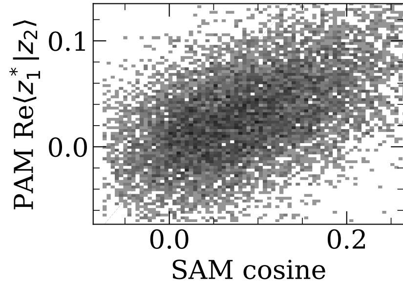
Synonyms (N=10256)
