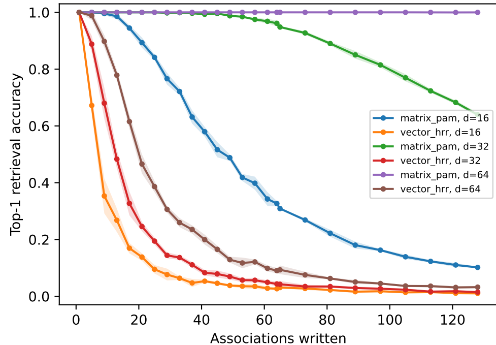
Equal embedding width
