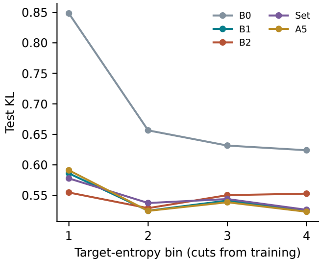
Entropy-stratified results
