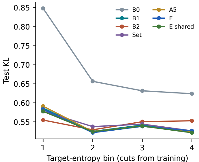
Entropy-stratified results
