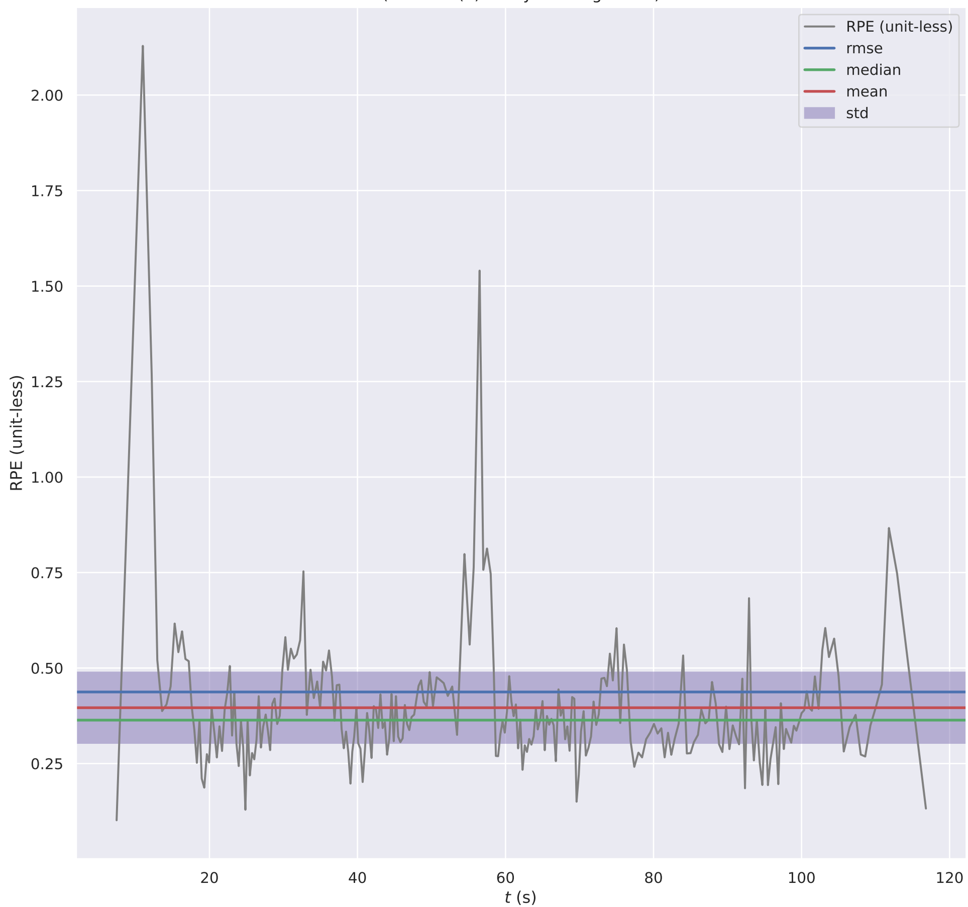
RPE w.r.t. full transformation (unit-less) for \delta = 1.0 (m) using consecutive pairs (with Sim(3) Umeyama alignment)
