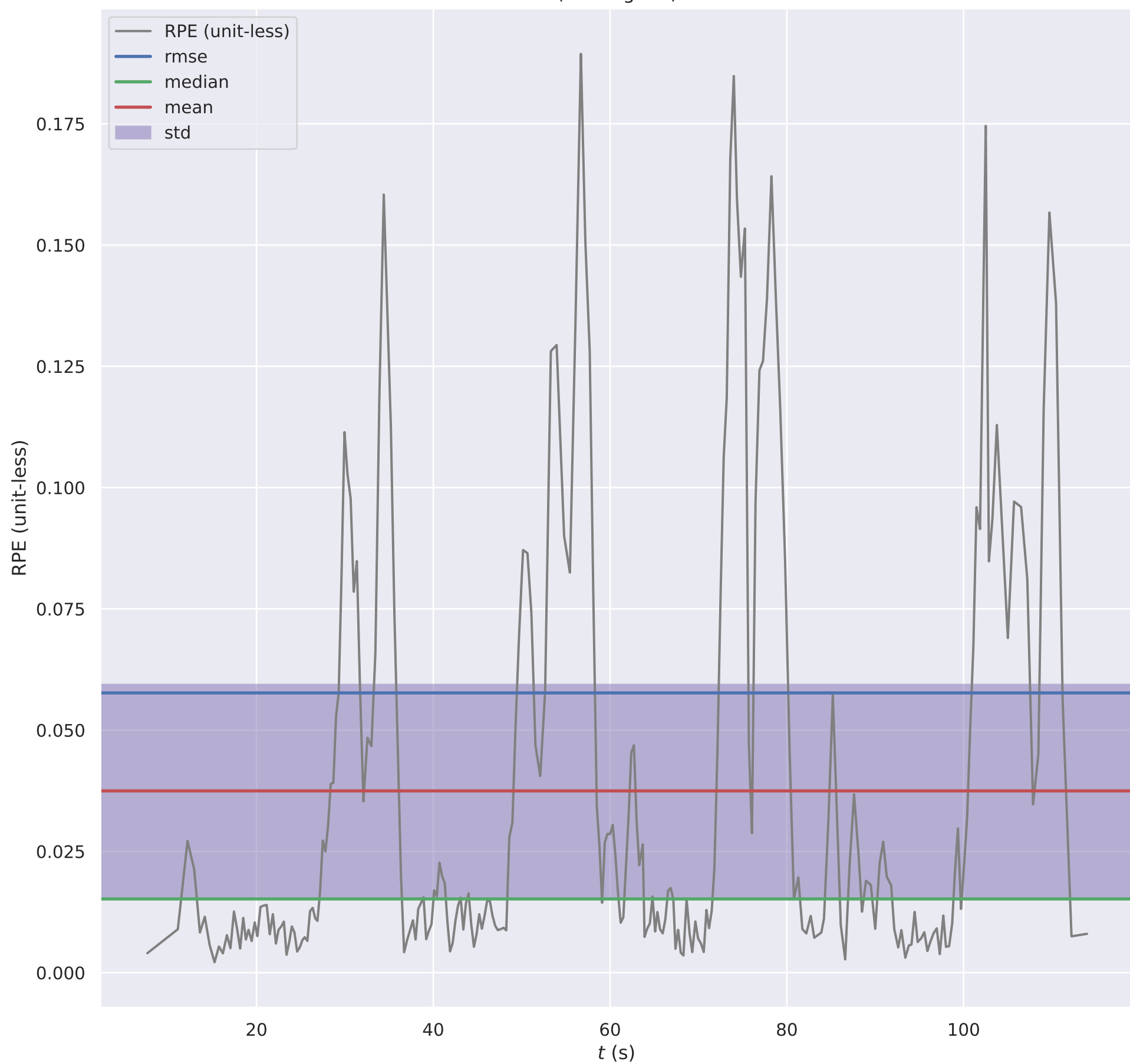
RPE w.r.t. rotation part (unit-less) for \delta = 1.0 (m) using consecutive pairs (not aligned)
