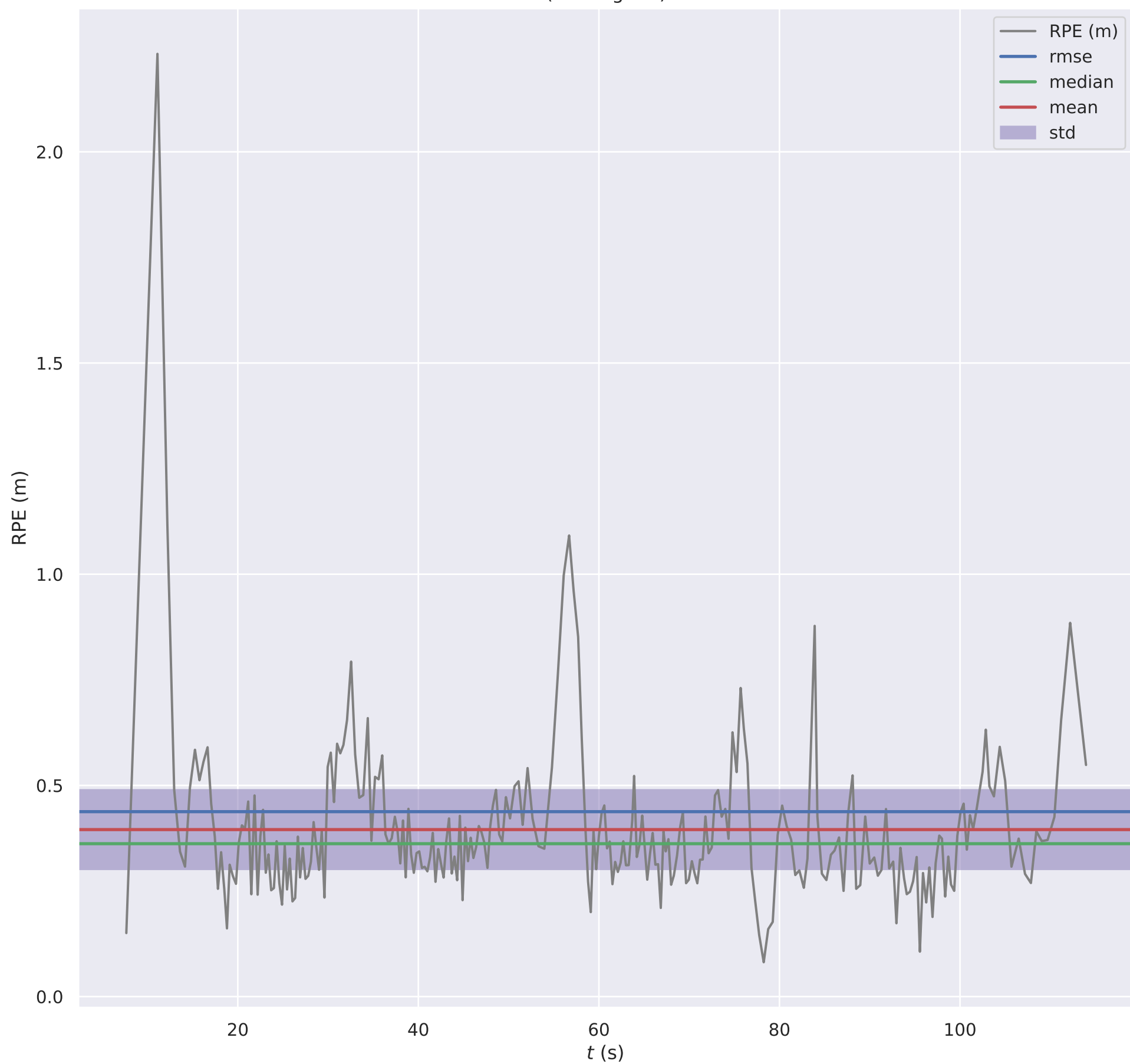
RPE w.r.t. translation part (m) for \delta = 1.0 (m) using consecutive pairs (not aligned)
