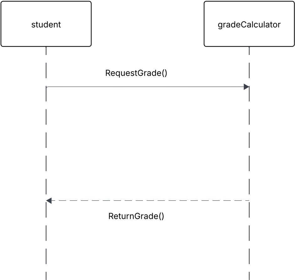
Sequence Diagram
