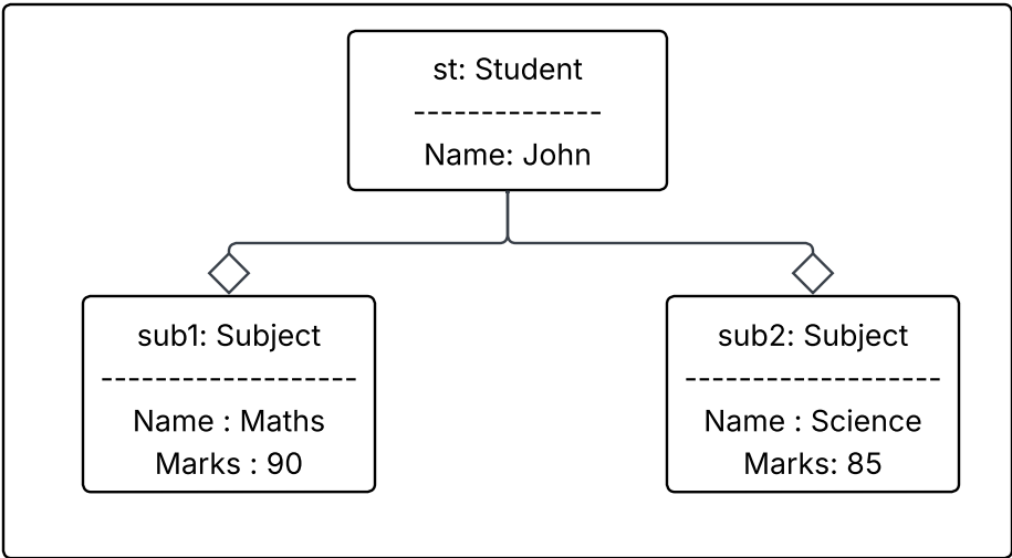
Object Diagram
