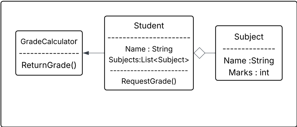
Class Diagram
