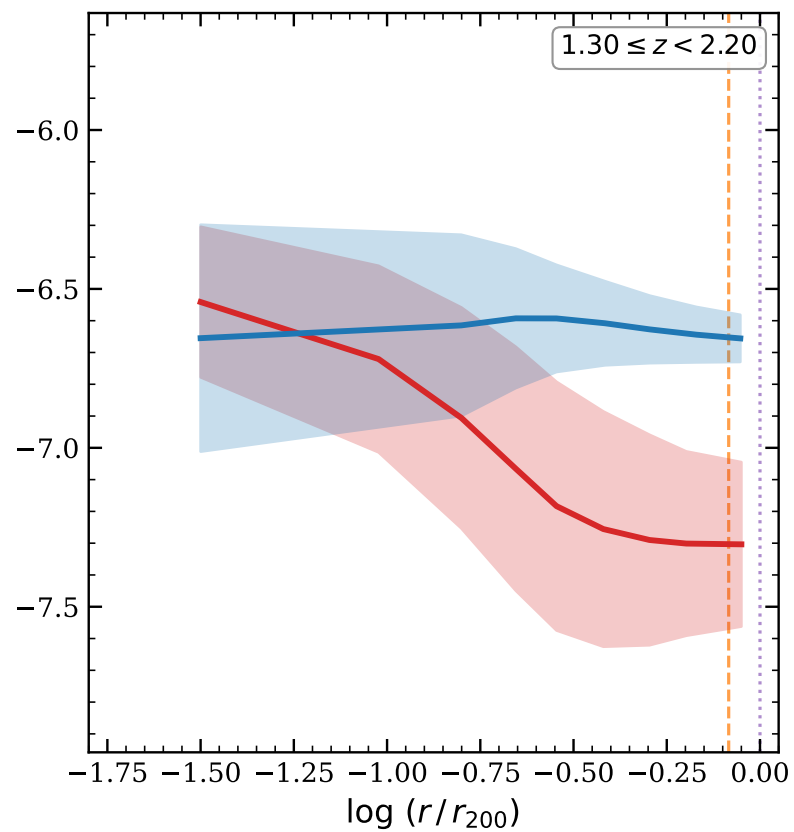
Average X-ray surface brightness profiles — CW-All Blue: X-ray detected Red: non-detected
