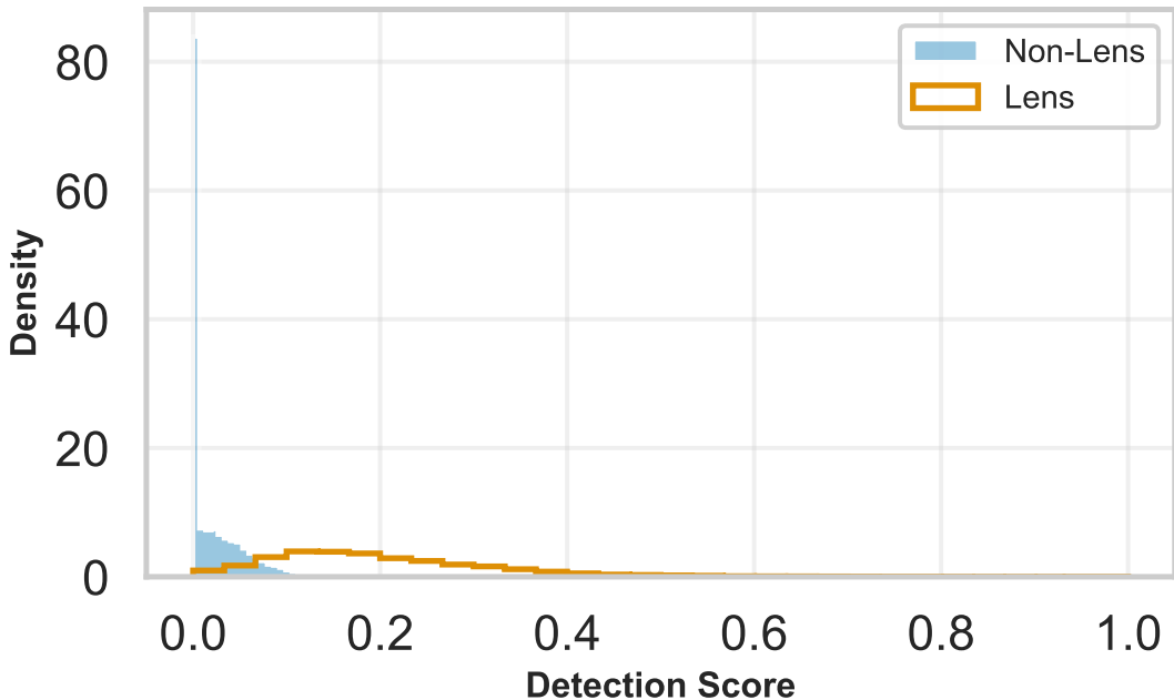
Custom20k_Empirical
