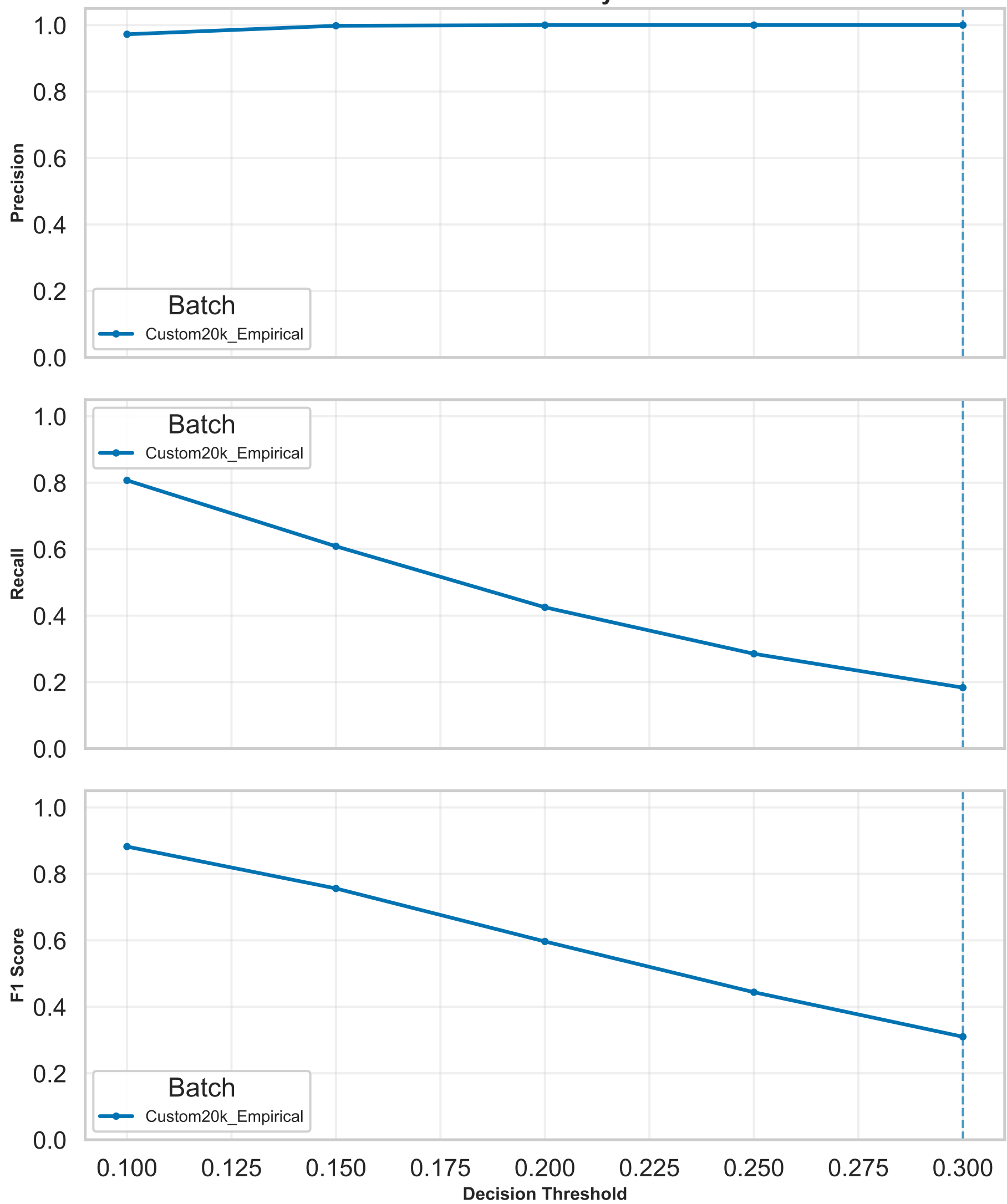
Threshold Summary Metrics
