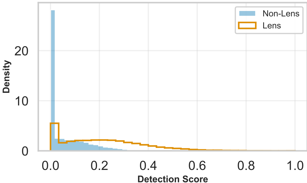
Custom20k
