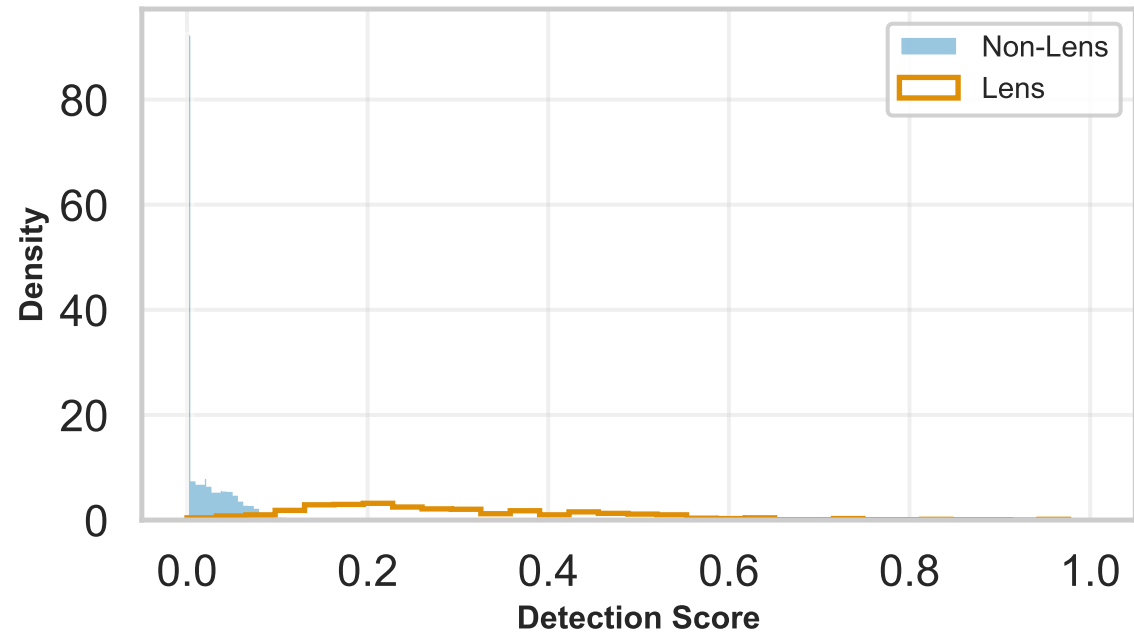
EmpiricalLatest
