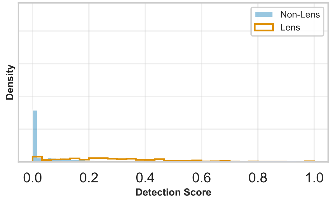
AblationLatest
