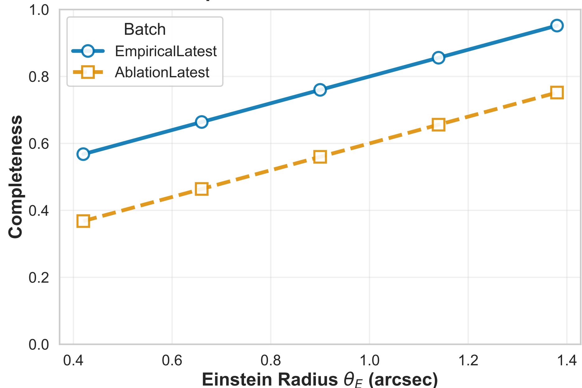
Completeness vs Einstein Radius
