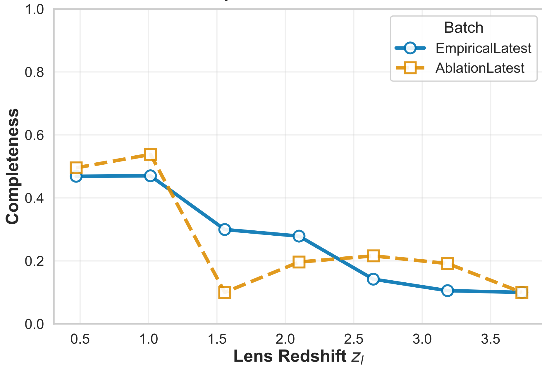
Completeness vs Redshift
