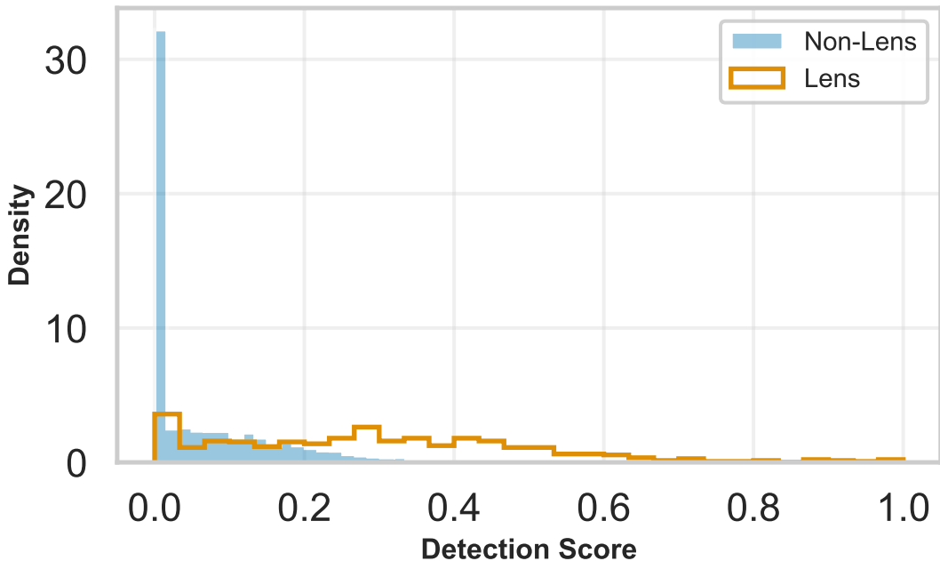
AblationLatest
