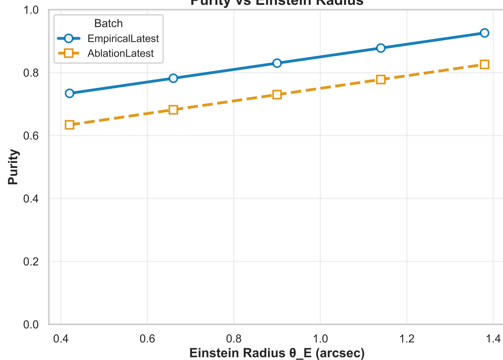
Purity vs Einstein Radius
