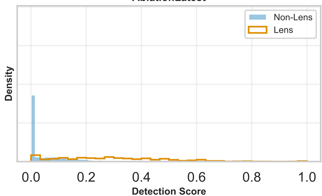
AblationLatest
