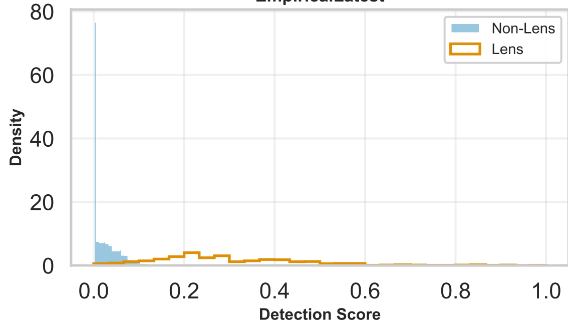
EmpiricalLatest
