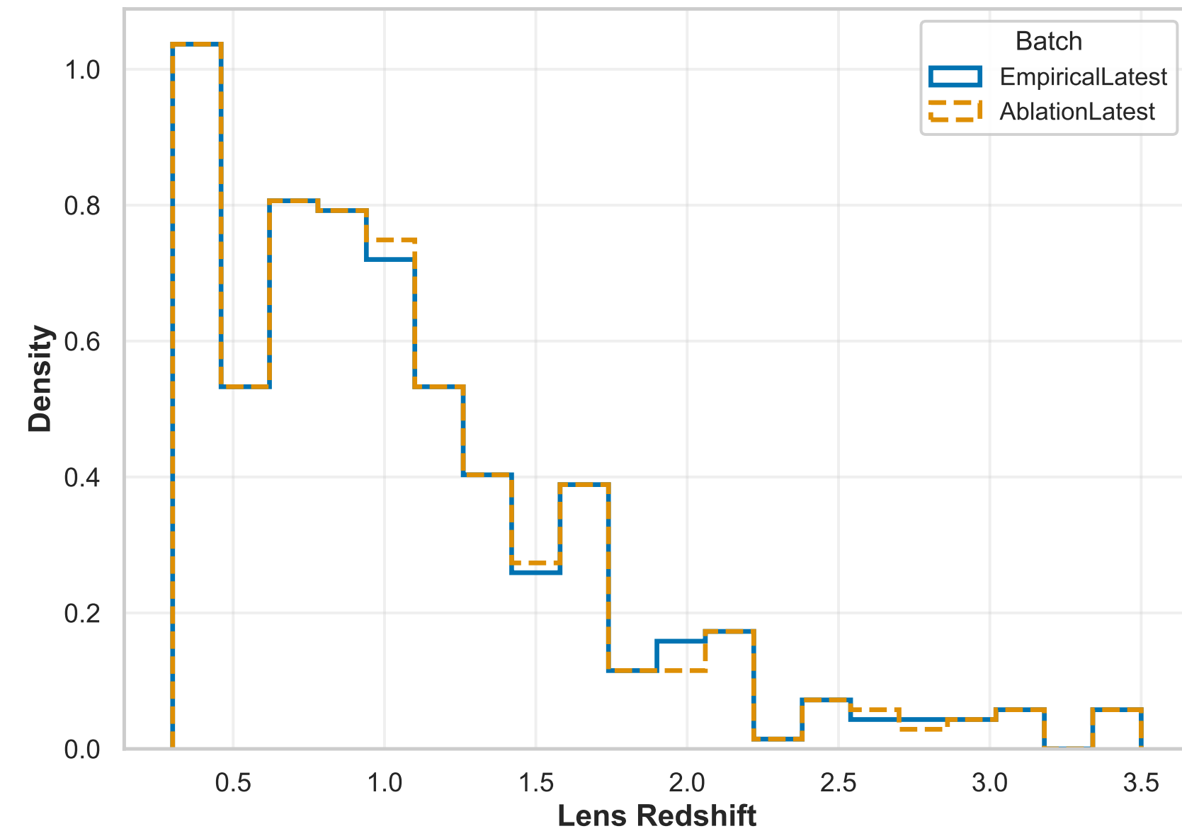
Lens Redshift Distribution
