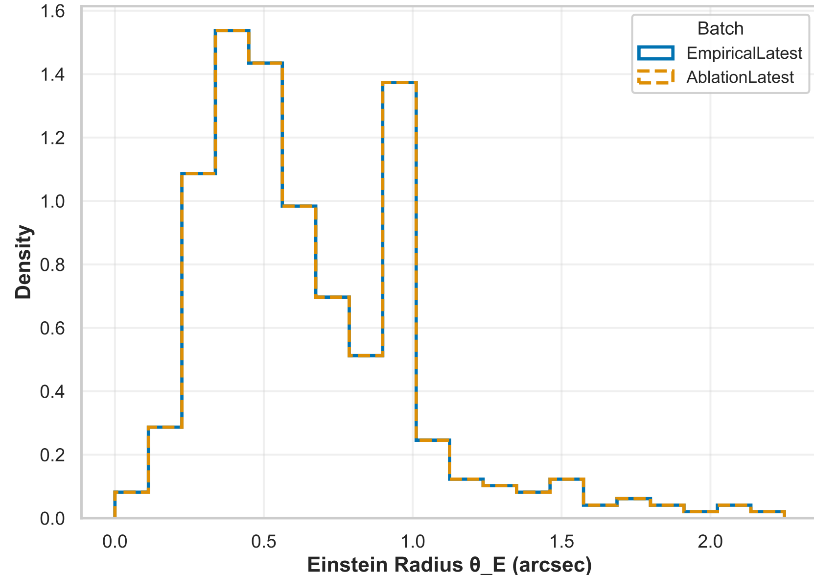
Einstein Radius Distribution
