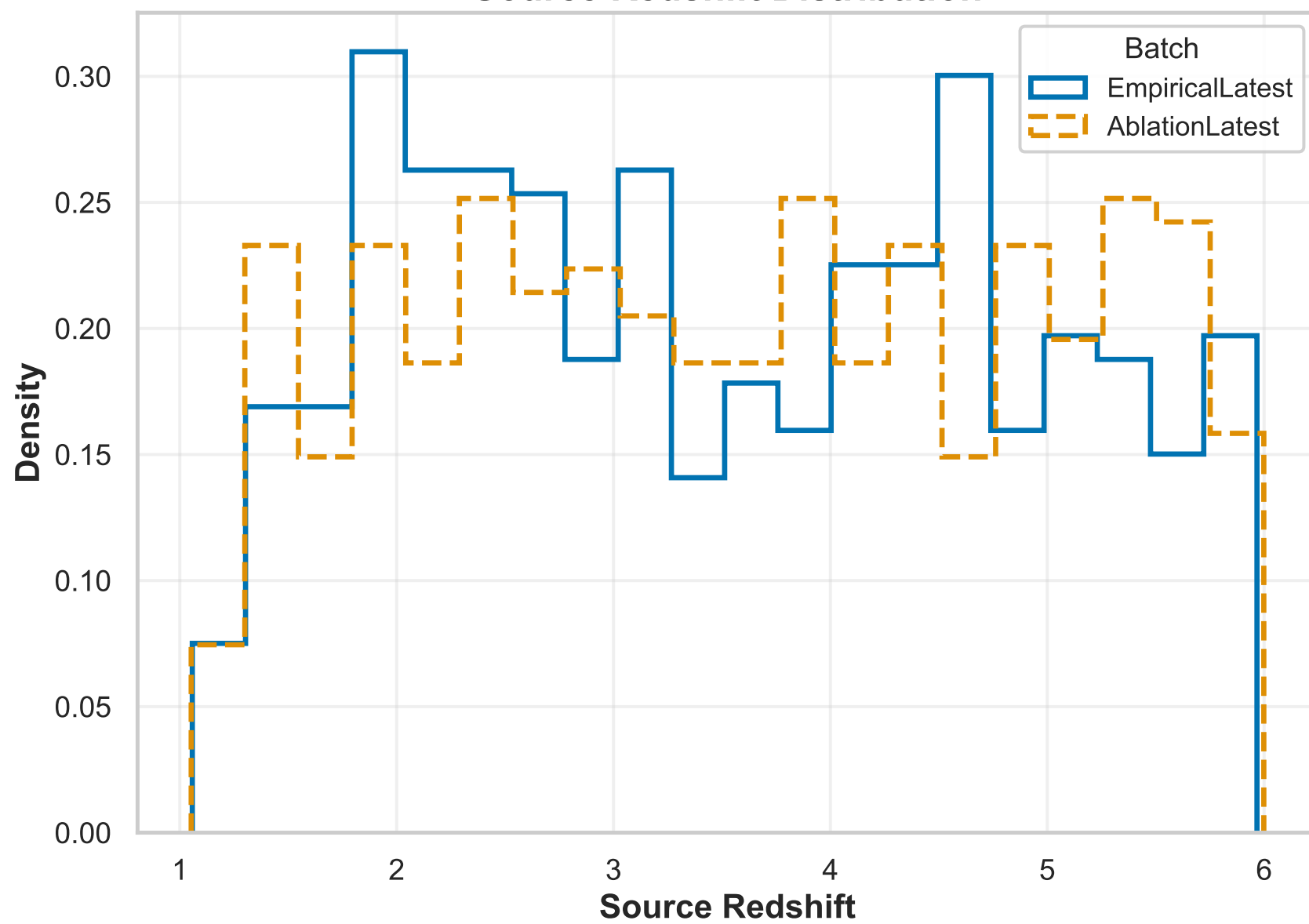
Source Redshift Distribution
