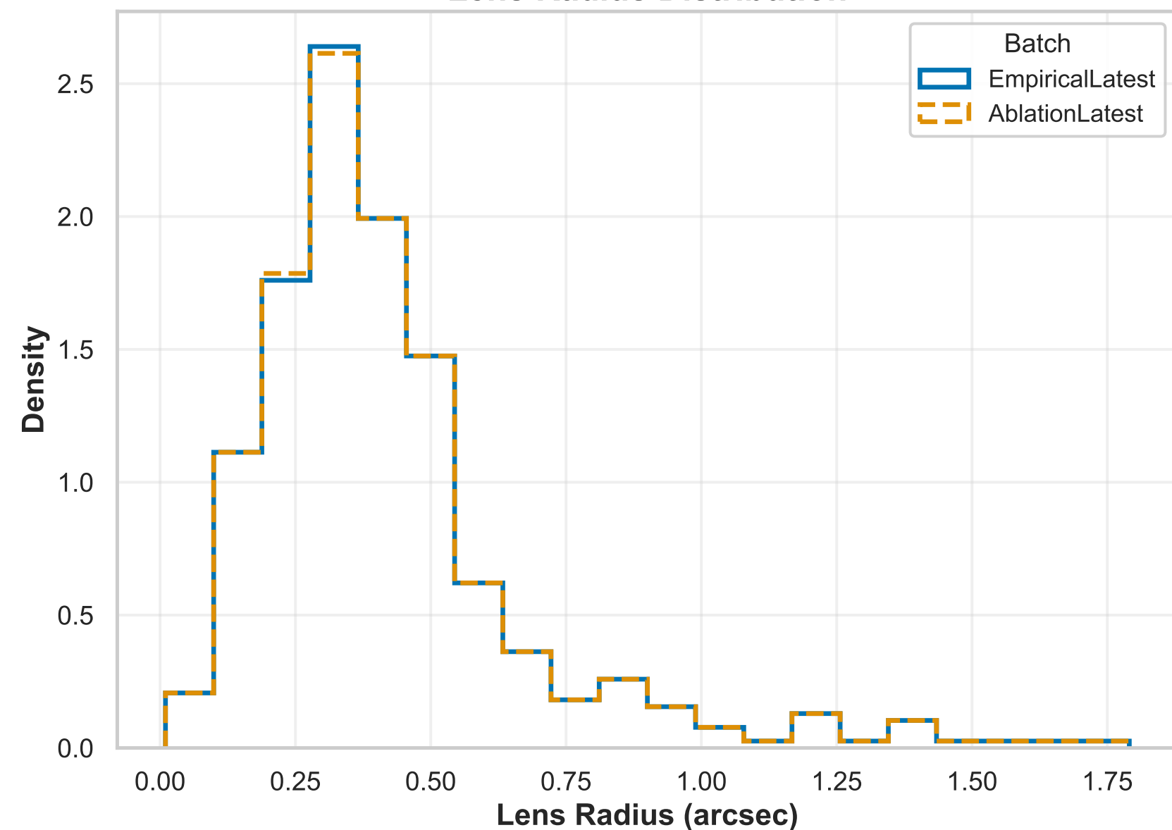
Lens Radius Distribution
