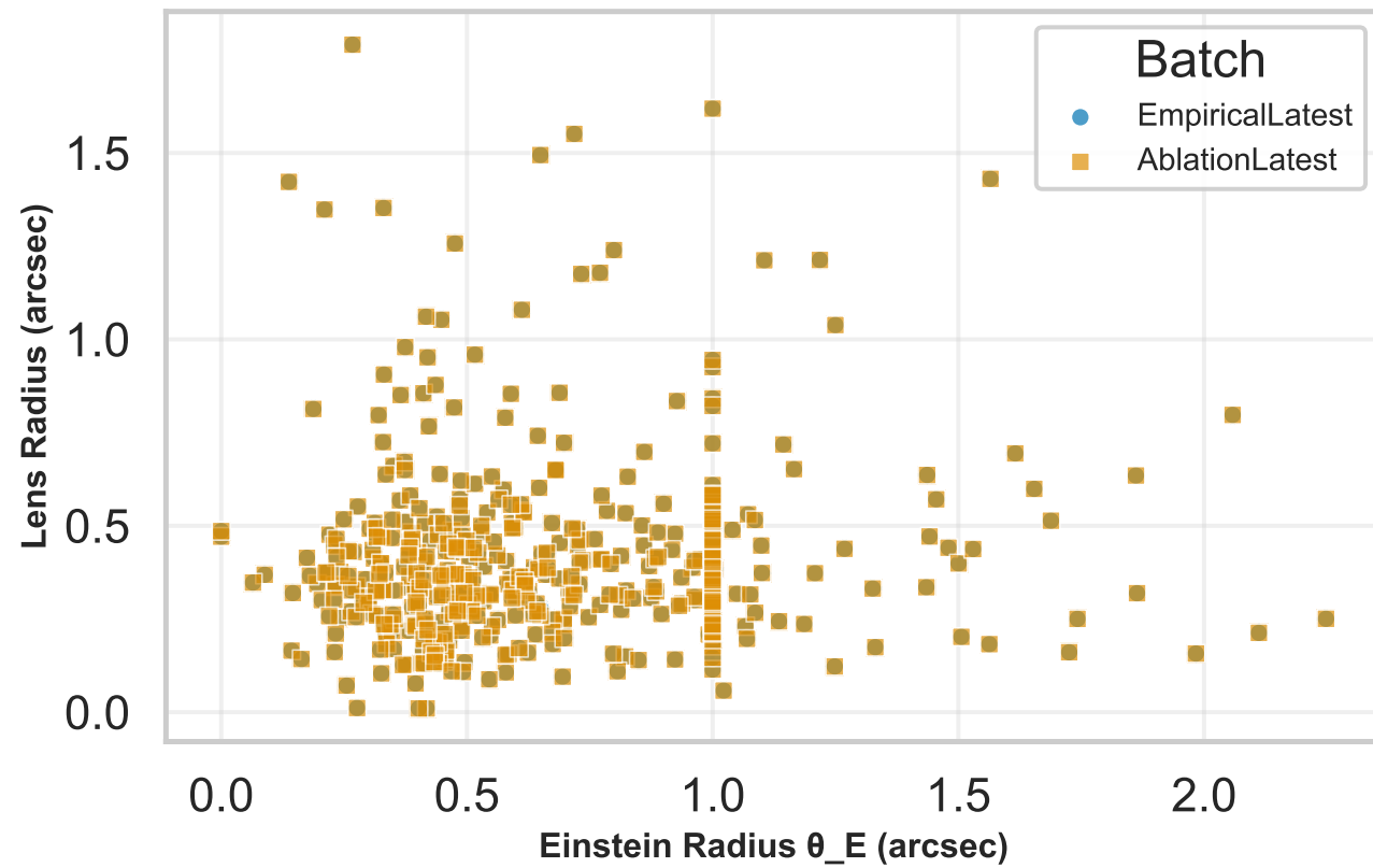
Lens Radius vs Einstein Radius
