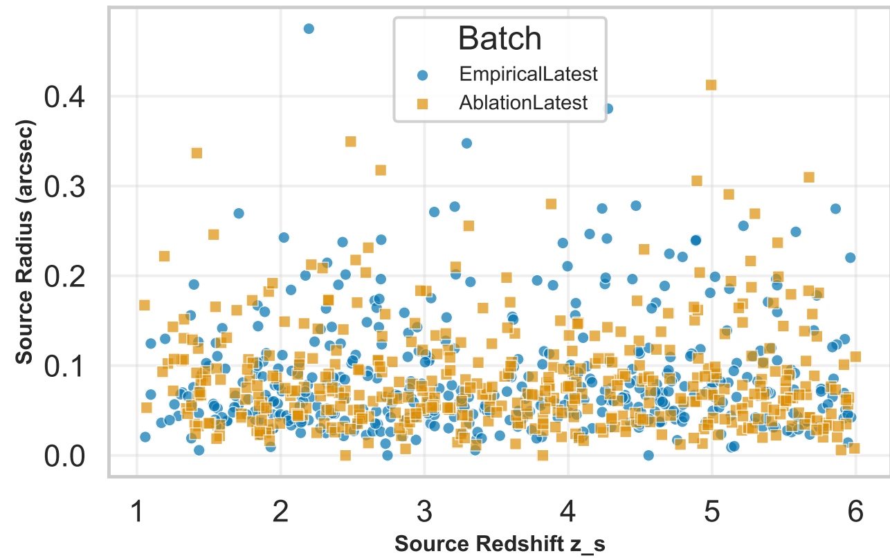
Source Size vs Redshift
