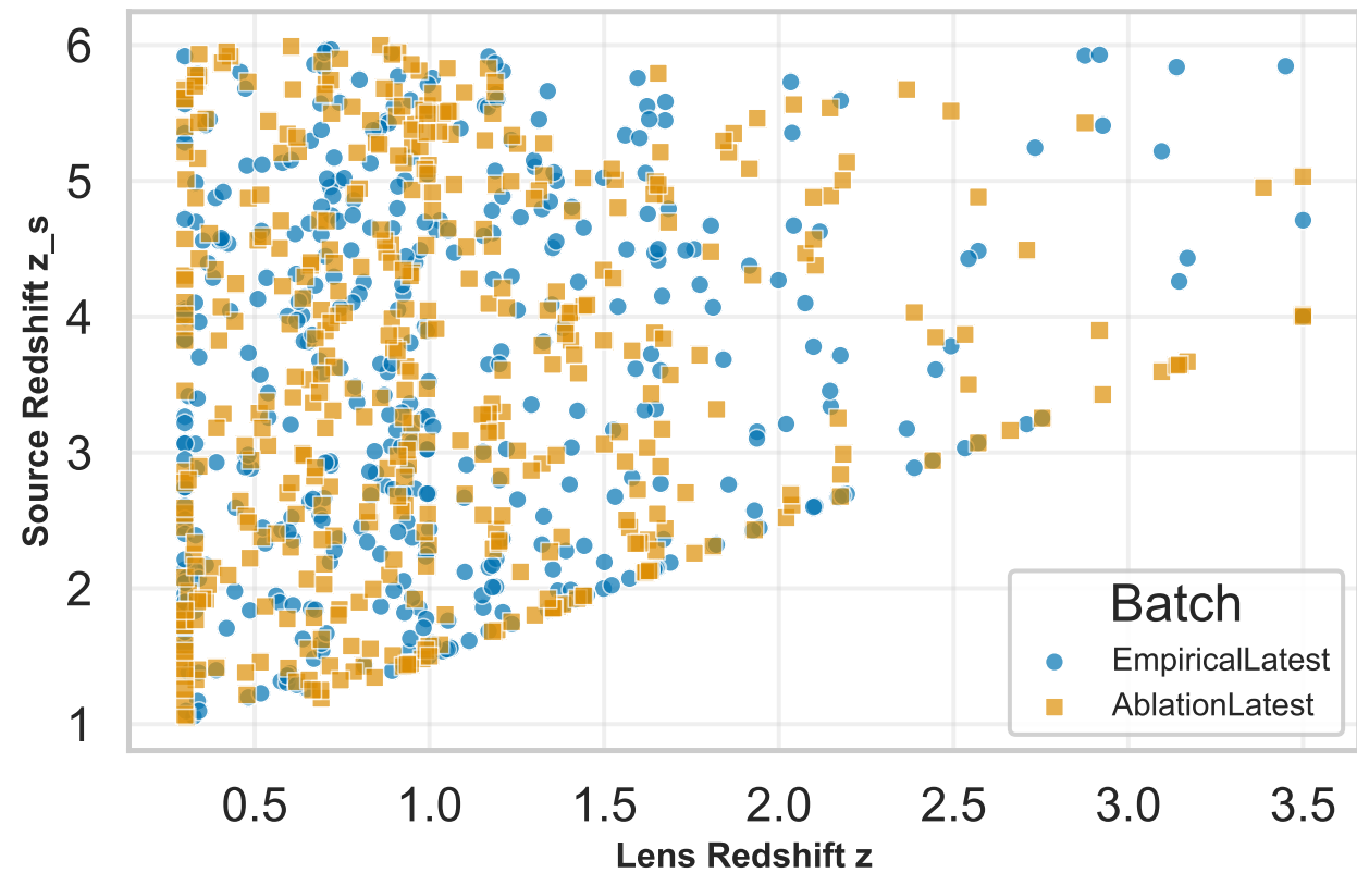
Source vs Lens Redshift
