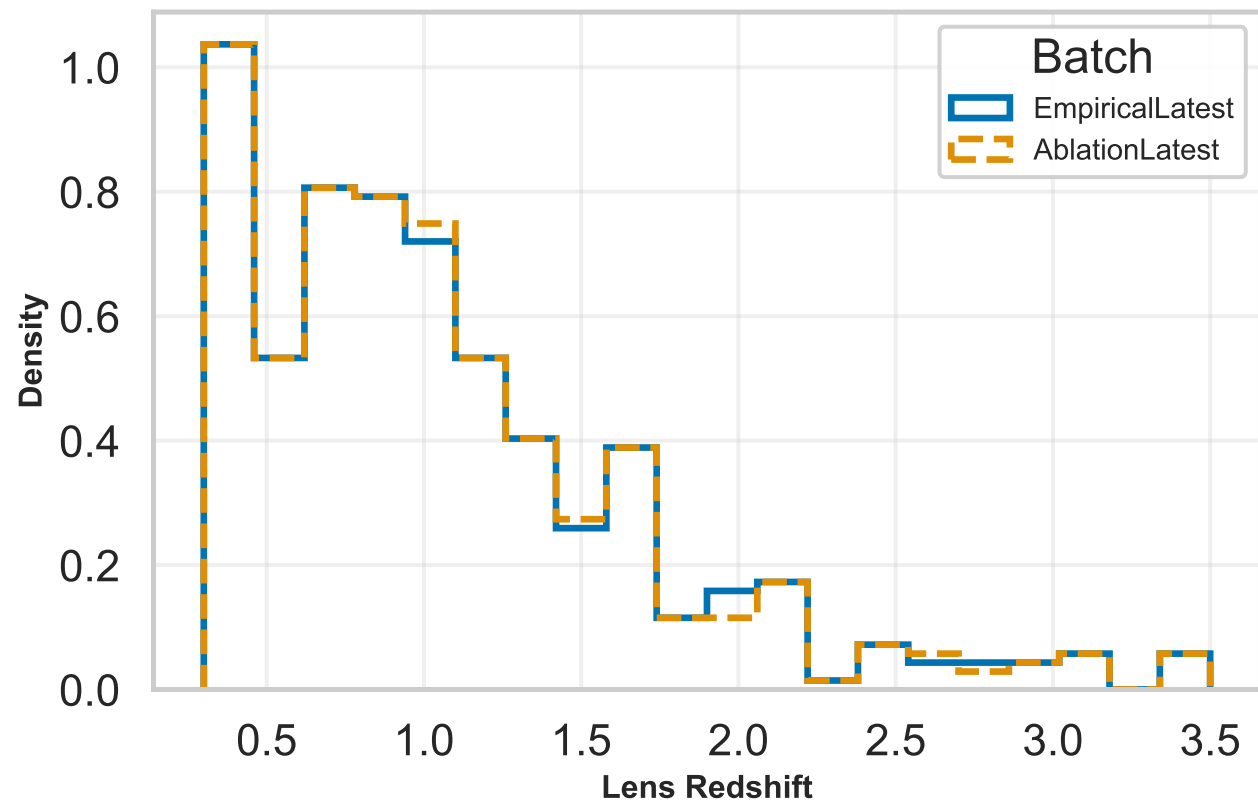
Lens Redshift Distribution
