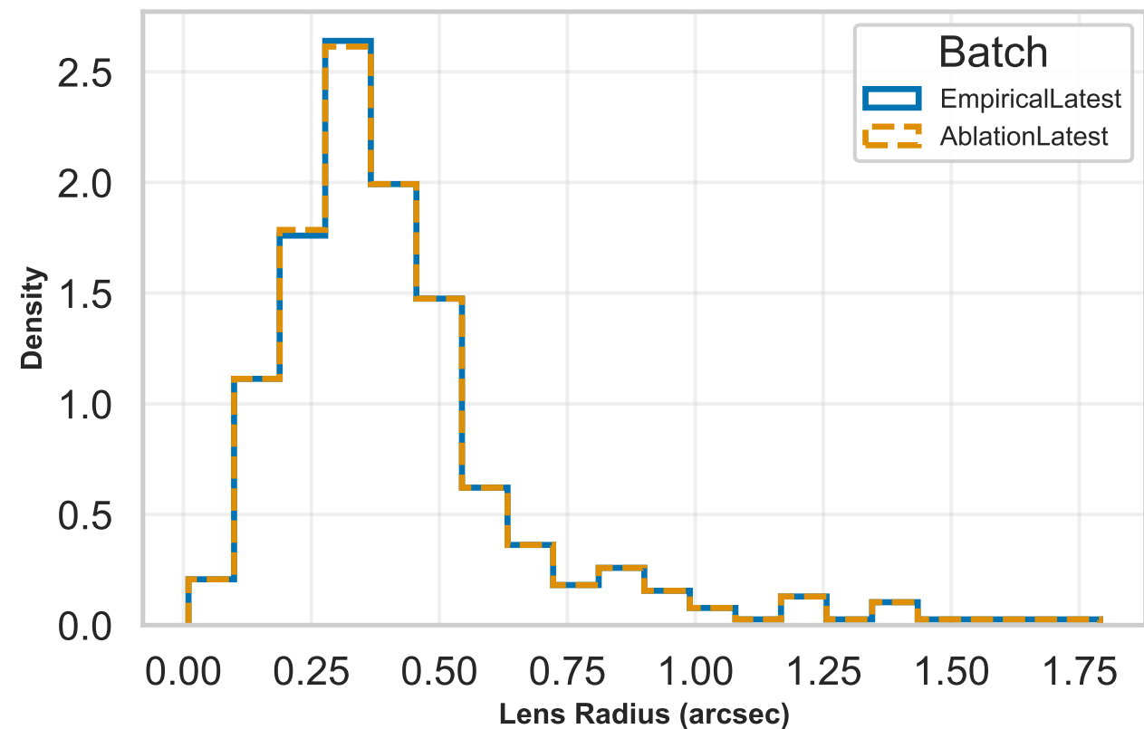
Lens Radius Distribution
