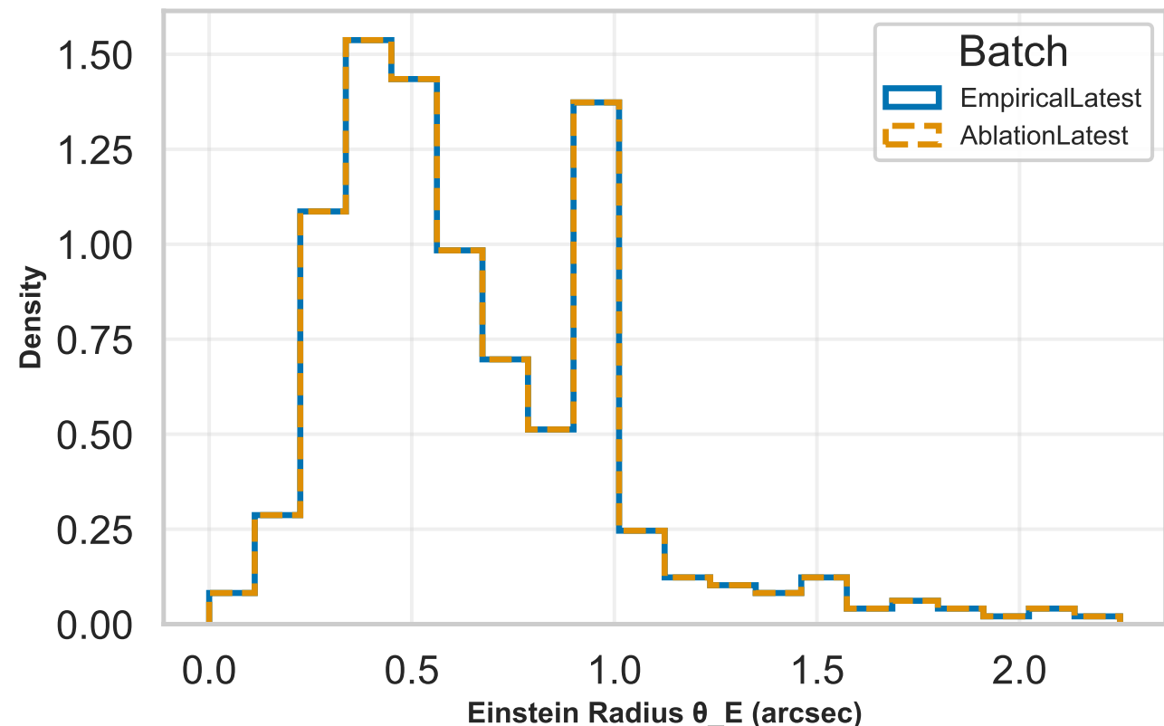
Einstein Radius Distribution
