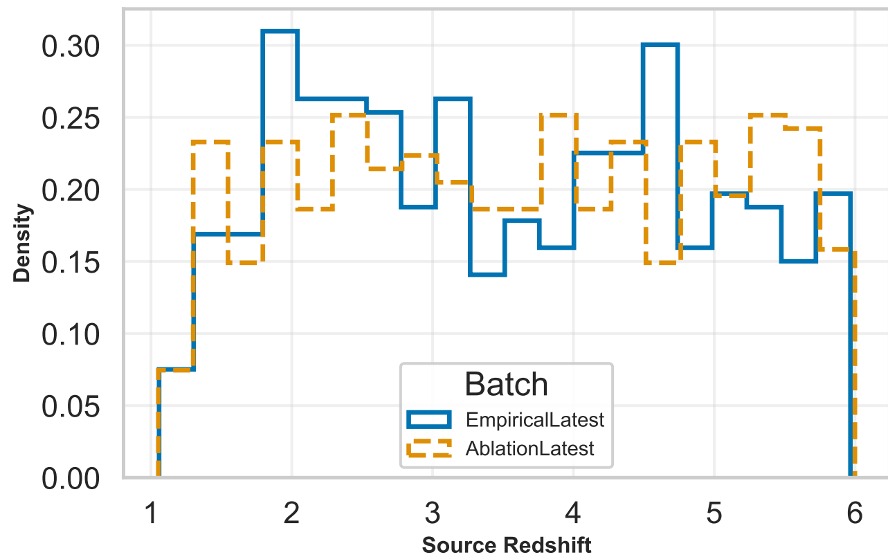
Source Redshift Distribution
