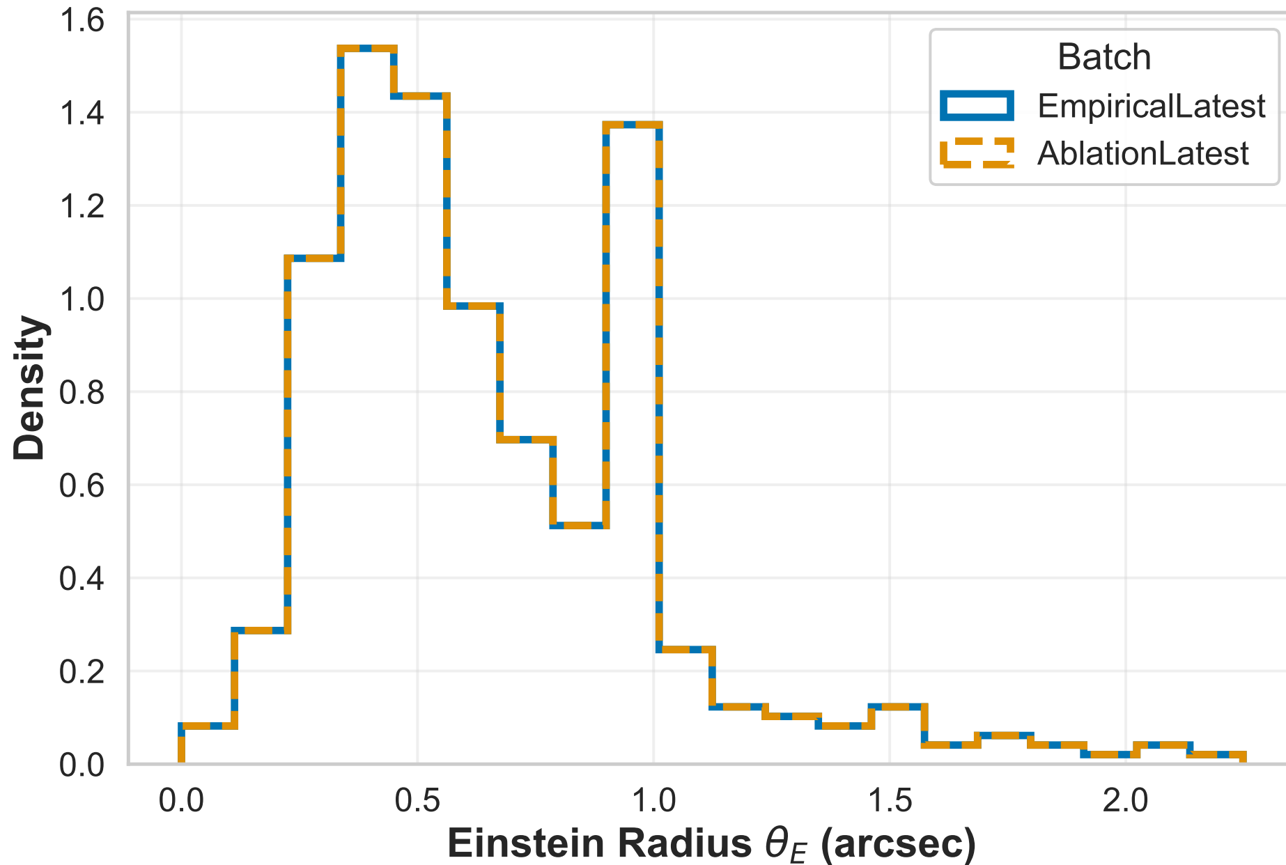
Einstein Radius Distribution
