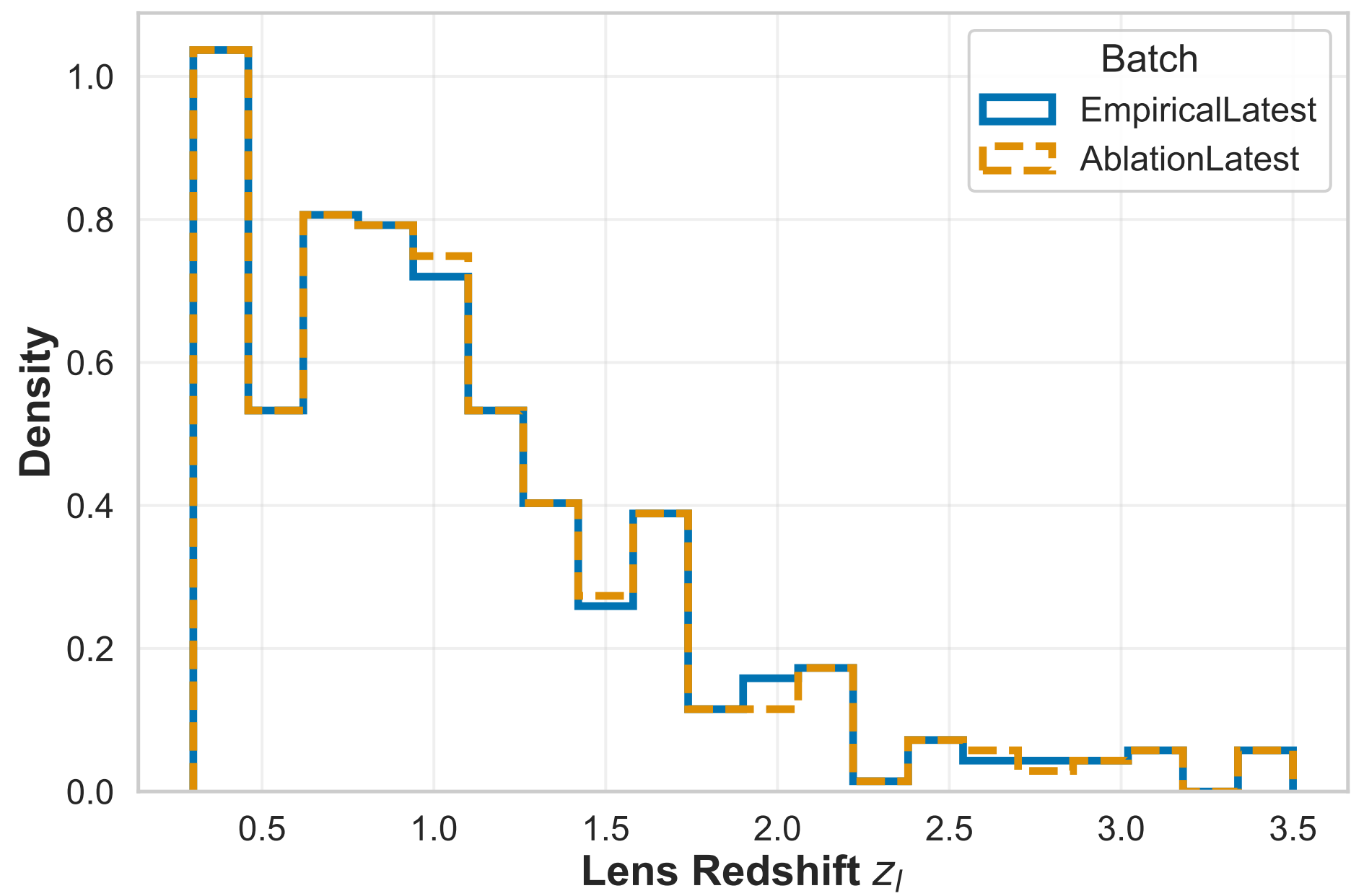
Lens Redshift Distribution
