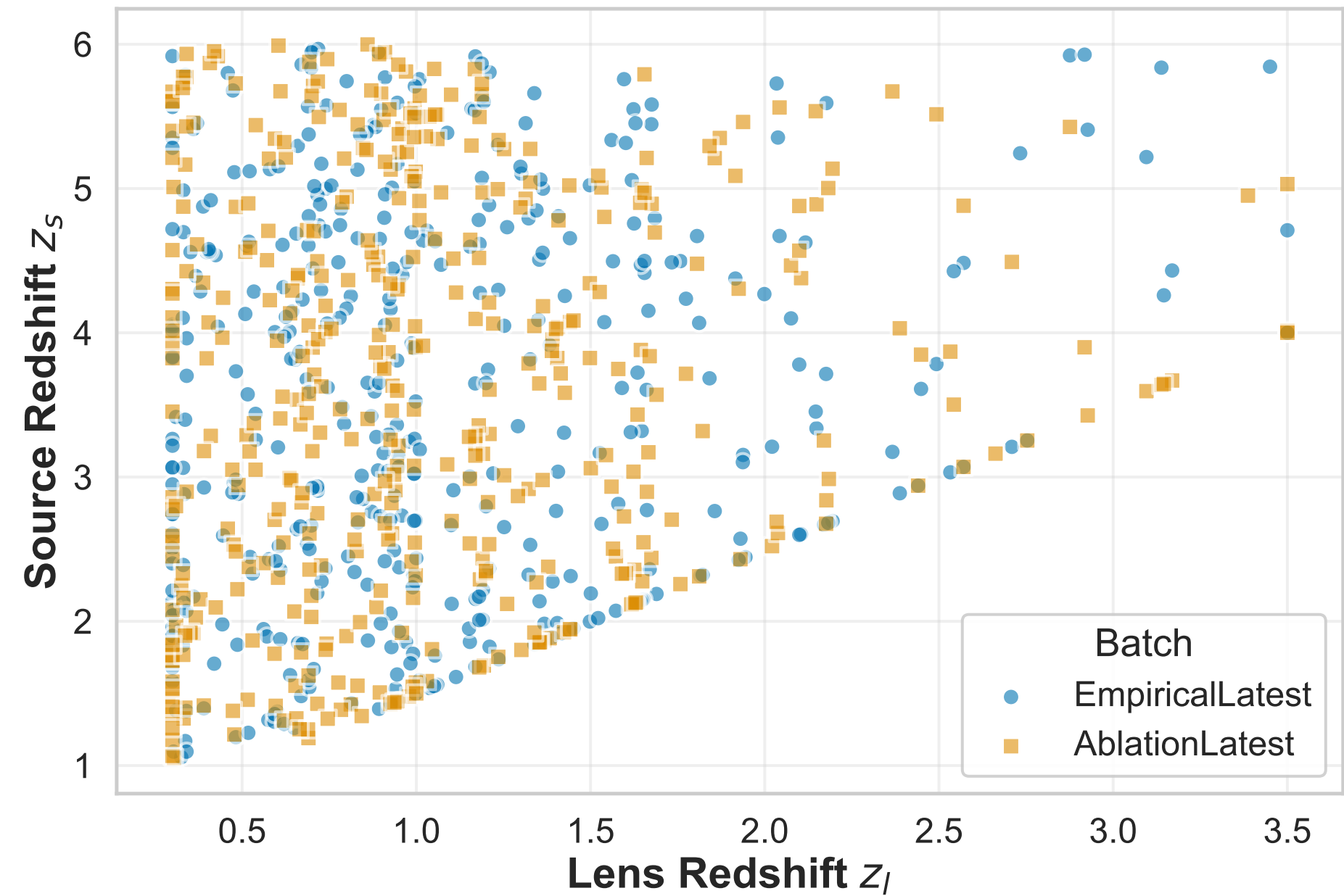
Source vs Lens Redshift
