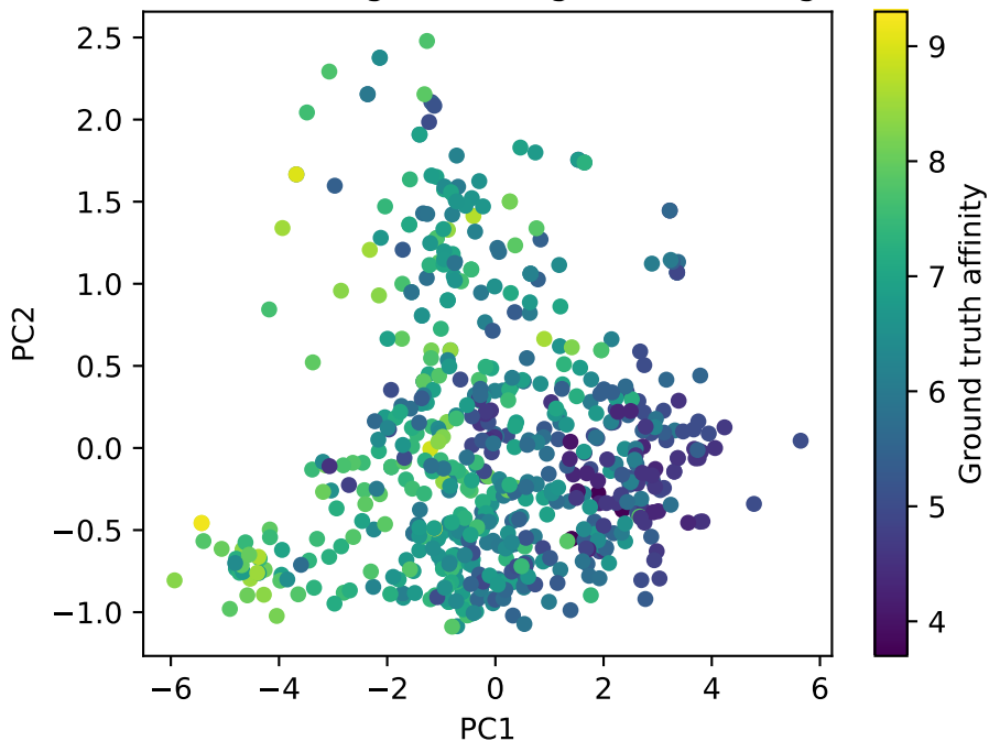
Test embeddings (PCA) - ground truth (gat)
