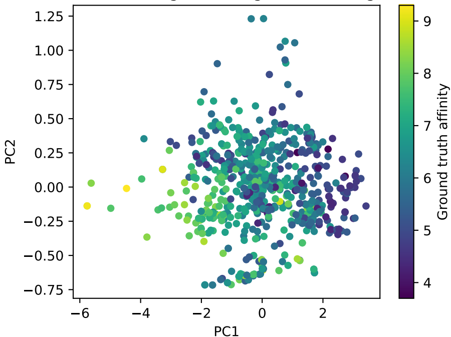
Test embeddings (PCA) - ground truth (gcn)
