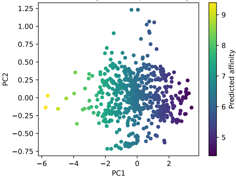
Test embeddings (PCA) - predicted (gcn)
