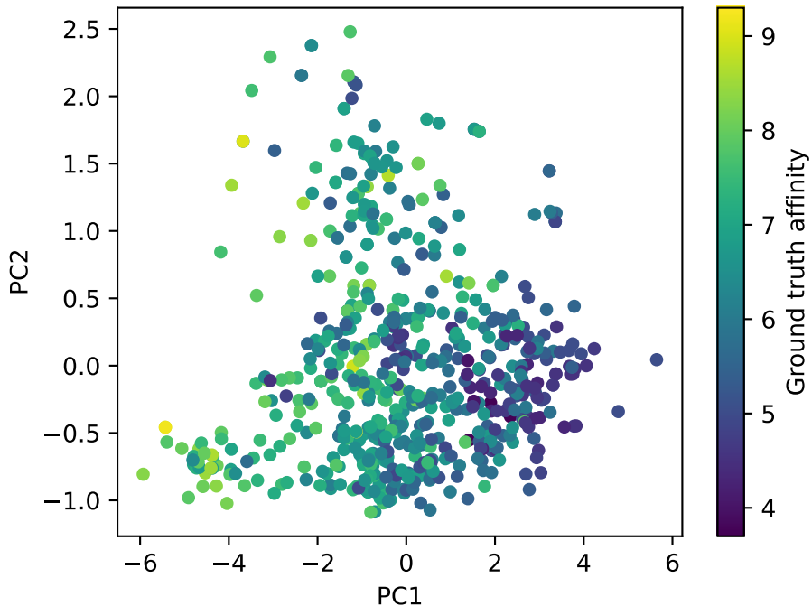
Test embeddings (PCA) - ground truth (gin)
