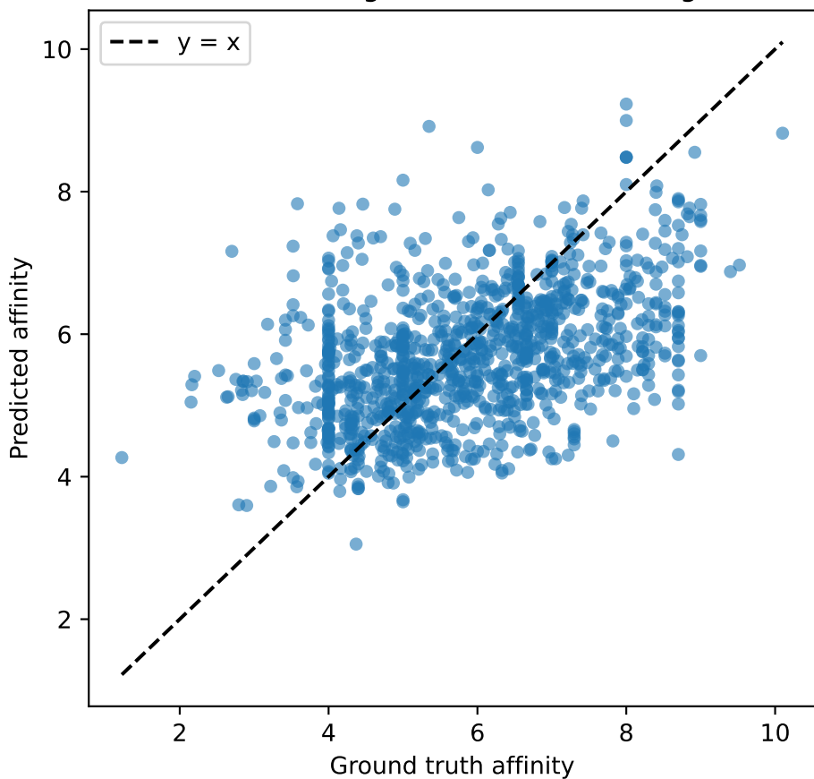
Predicted vs ground truth - test (sage)
