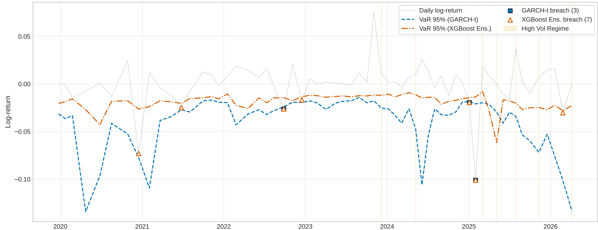
FIBRA Index — 95% VaR Backtest: GARCH-t vs. XGBoost Ensemble
