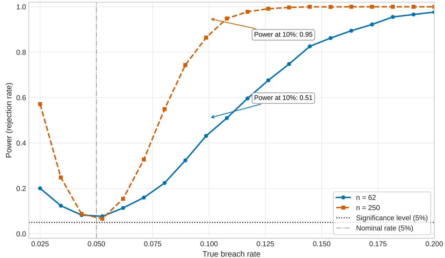
Kupiec POF Test — Power Curve
