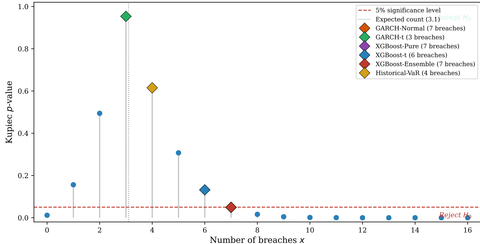
Kupiec POF Test: p -value Staircase ( n = 62 , \alpha = 0.05 )
