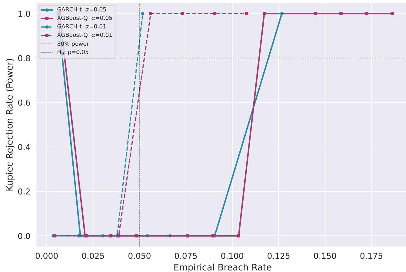
Empirical Power Curve — n=58
