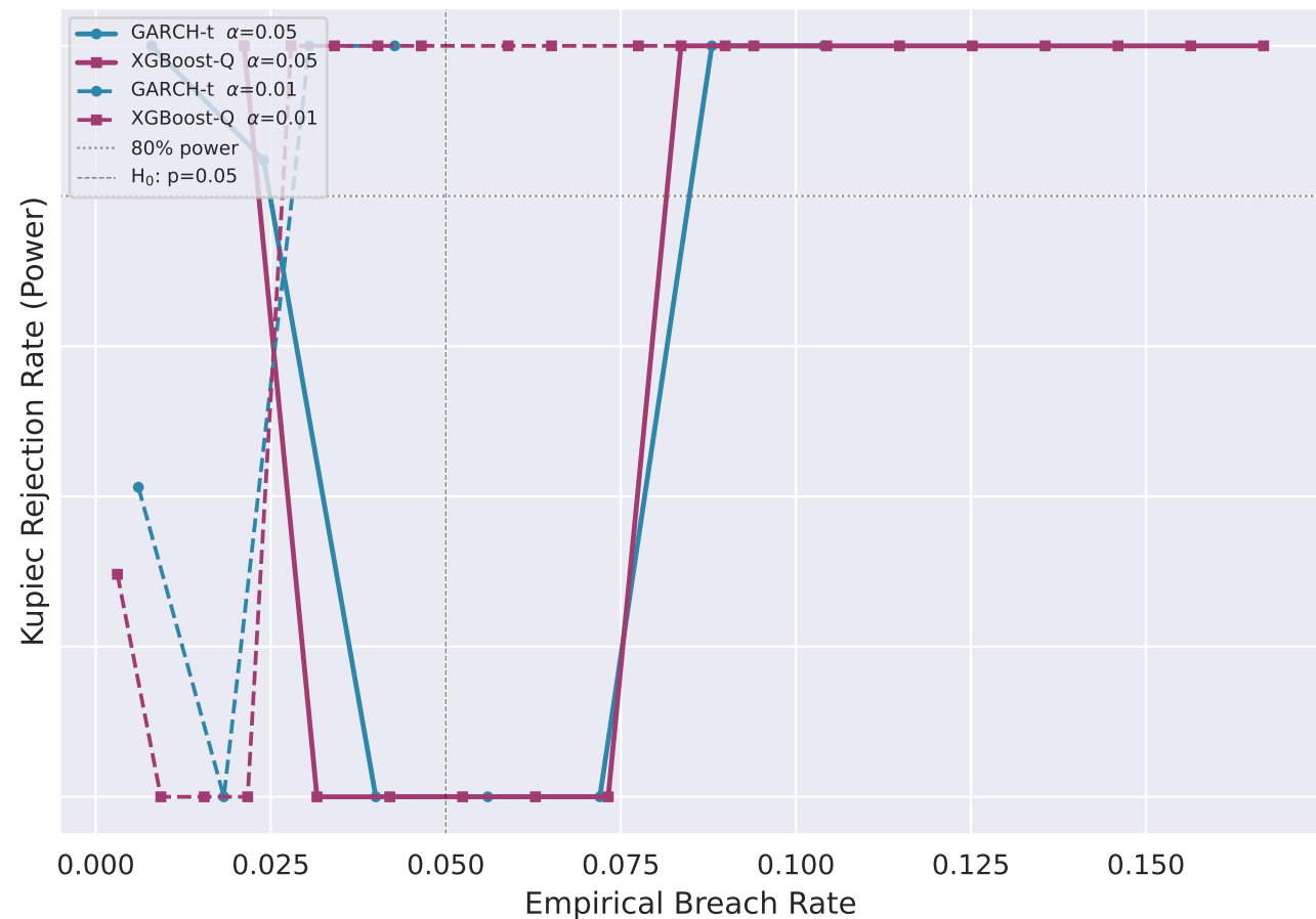
Empirical Power Curve — n=250
