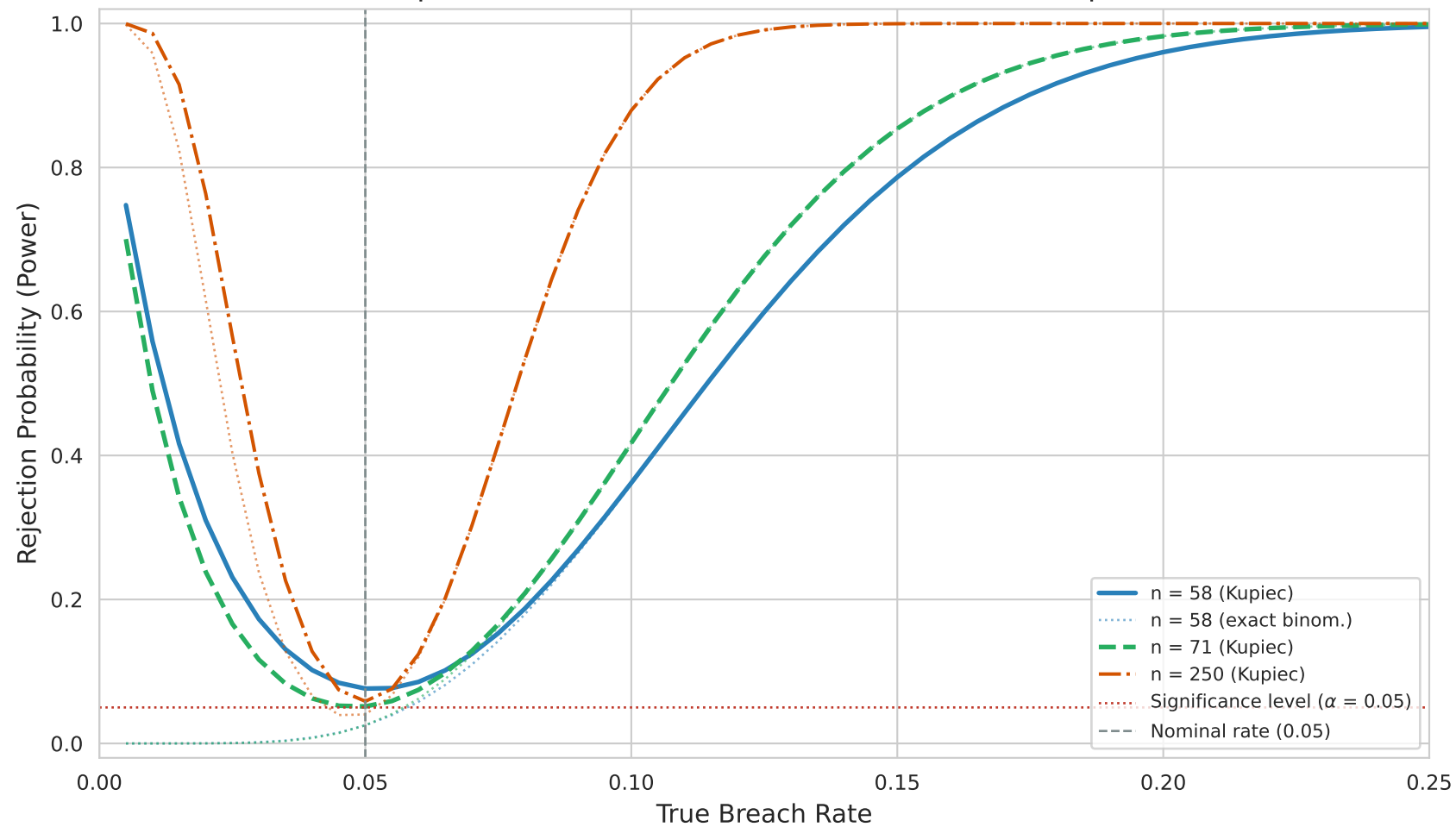
Kupiec POF Test — Power Curves for Small Samples
