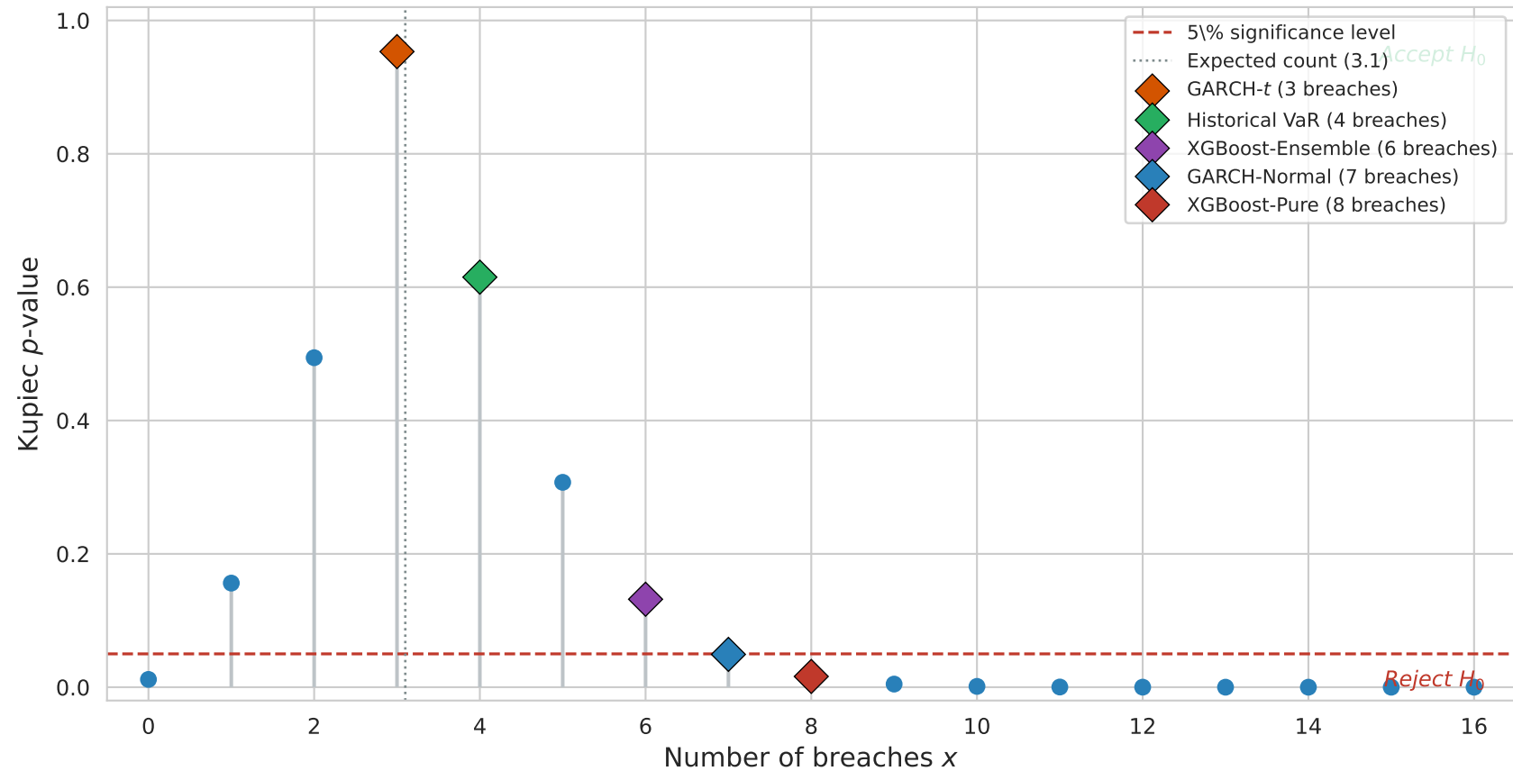
Kupiec POF Test: p -value Staircase ( n = 62, \alpha = 0.05 )
