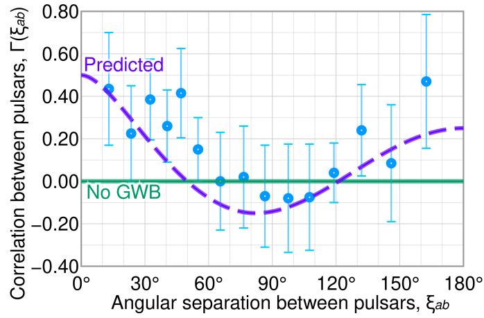
Figure 40: Plot of the correlations observed by NANOGrav (2023) vs angular separation between pulsars, compared with a theoretical model (dashed purple) and if there were no gravitational wave background (solid green) Credits: Wikipedia.
